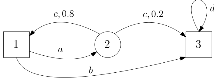
Figure 4.9 – Game with states \mathbf{S} = \{1, 2, 3\} and actions \mathbf{A} as defined above.
