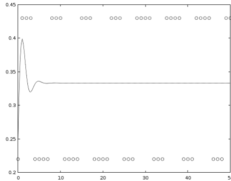
Figure 7.9 – Solid line represents \sum_{i=0}^k a_i(\delta) p_i^n and circles are in the upper side if \rho_{\delta_0}(n) = A and in the bottom if \rho_{\delta_0}(n) = B .
