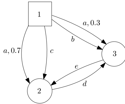
Figure 4.2 – A two-player stochastic arena
