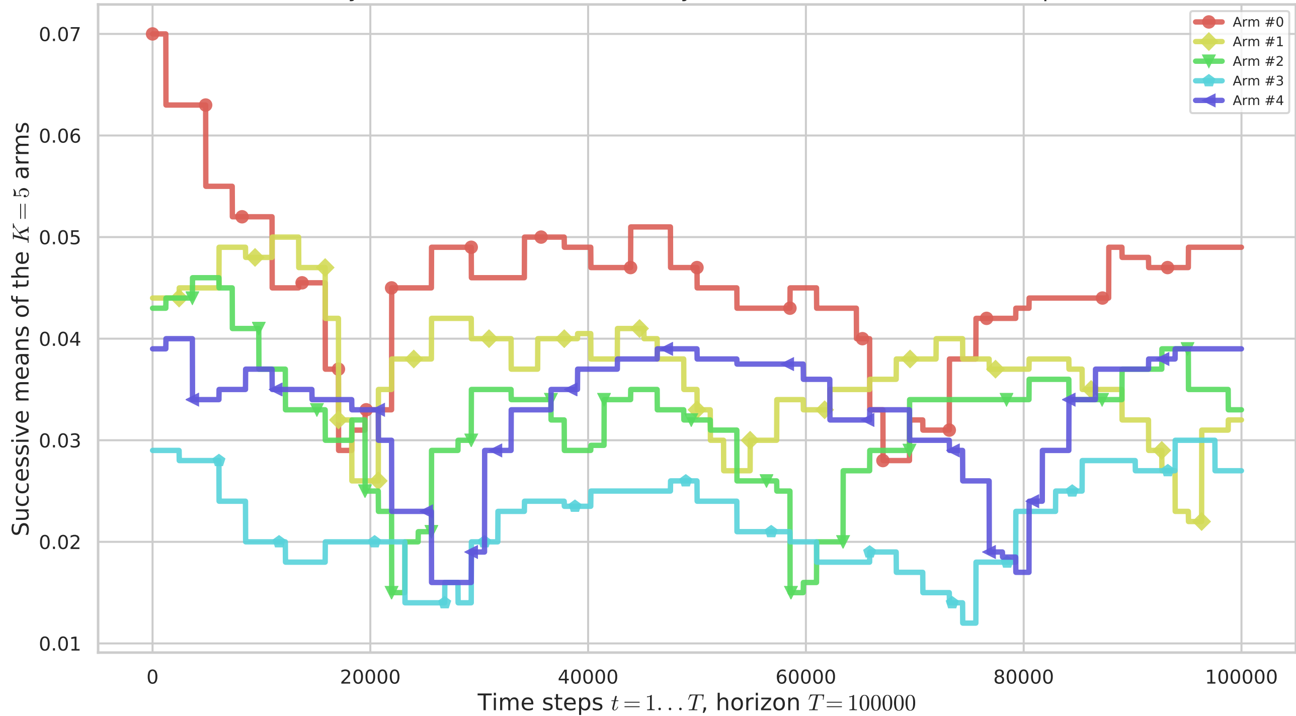
History of means for Non-Stationary MAB, Bernoulli with 81 break-points
