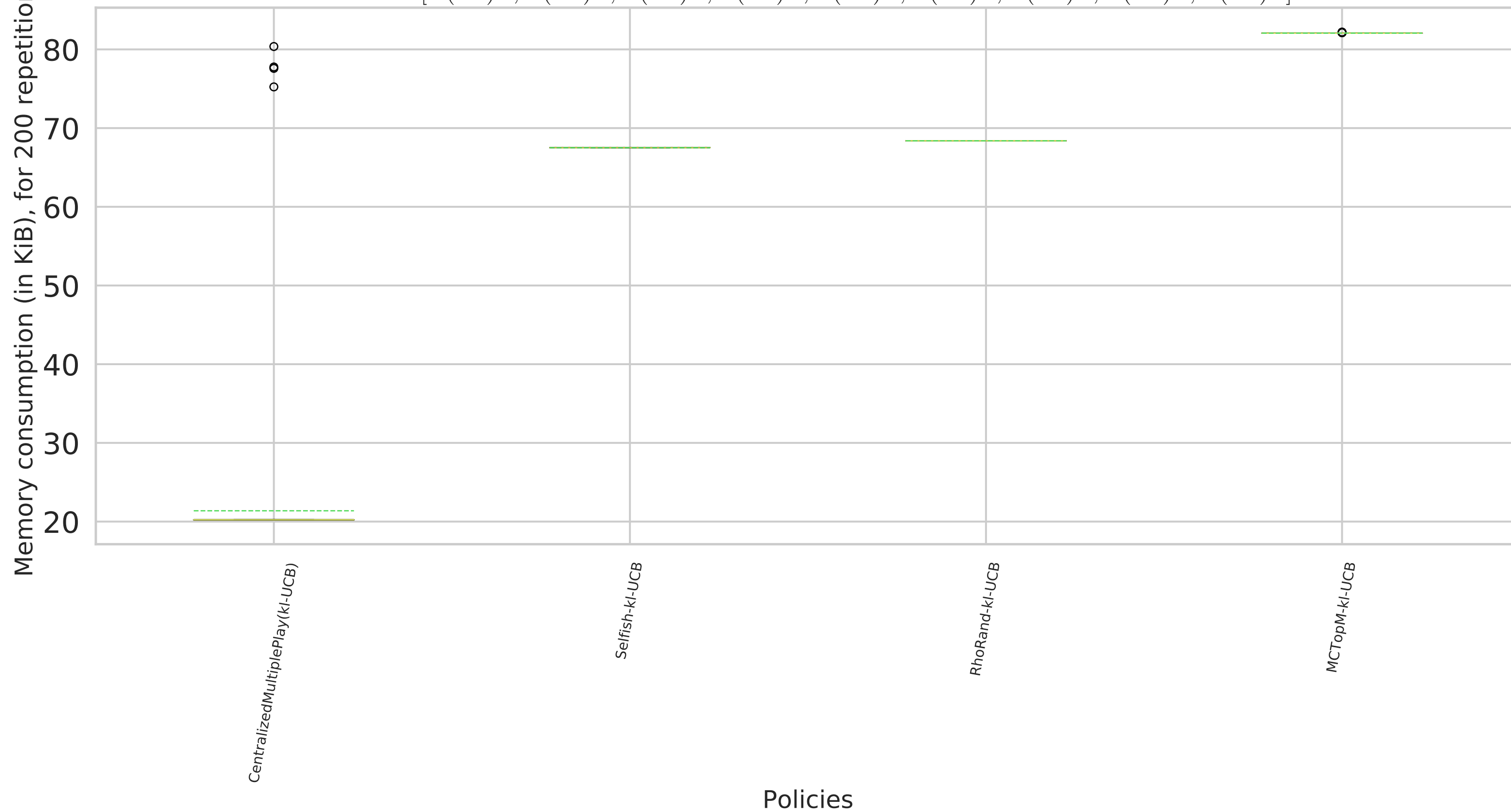
Memory consumption for different MP bandit algorithms, horizon T=10000 , averaged 200 times
