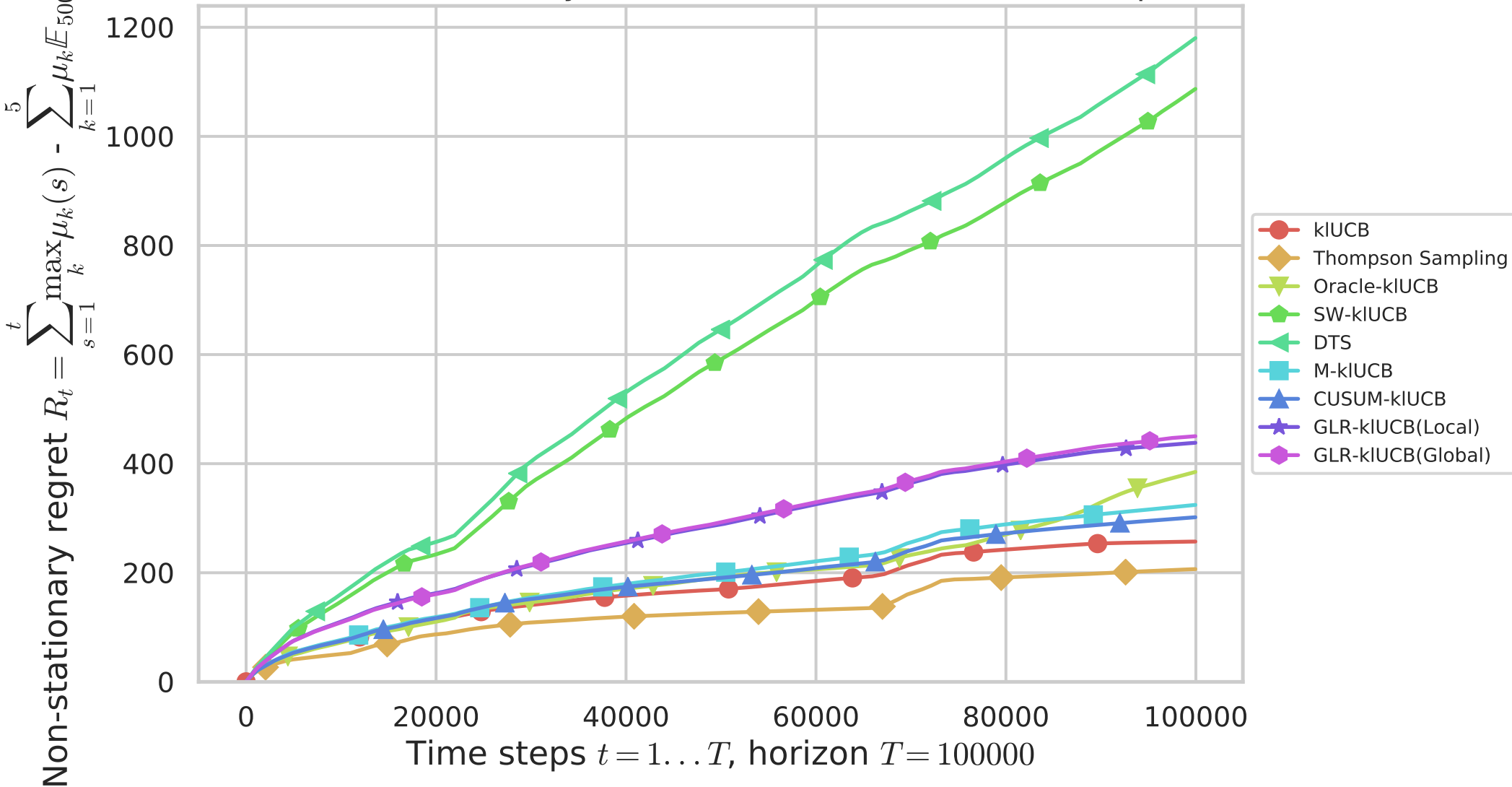
Cumulated regrets for different bandit algorithms, averaged 500 times 5 arms: Non-Stationary MAB, Bernoulli with \Upsilon = 81 break-points
