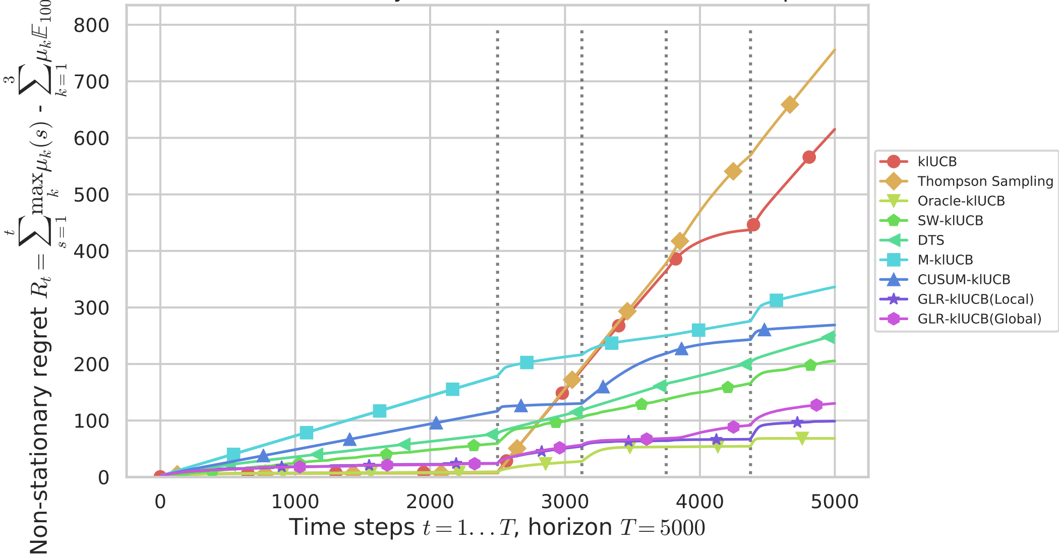
Cumulated regrets for different bandit algorithms, averaged 1000 times 3 arms: Non-Stationary MAB, Bernoulli with \Upsilon = 4 break-points
