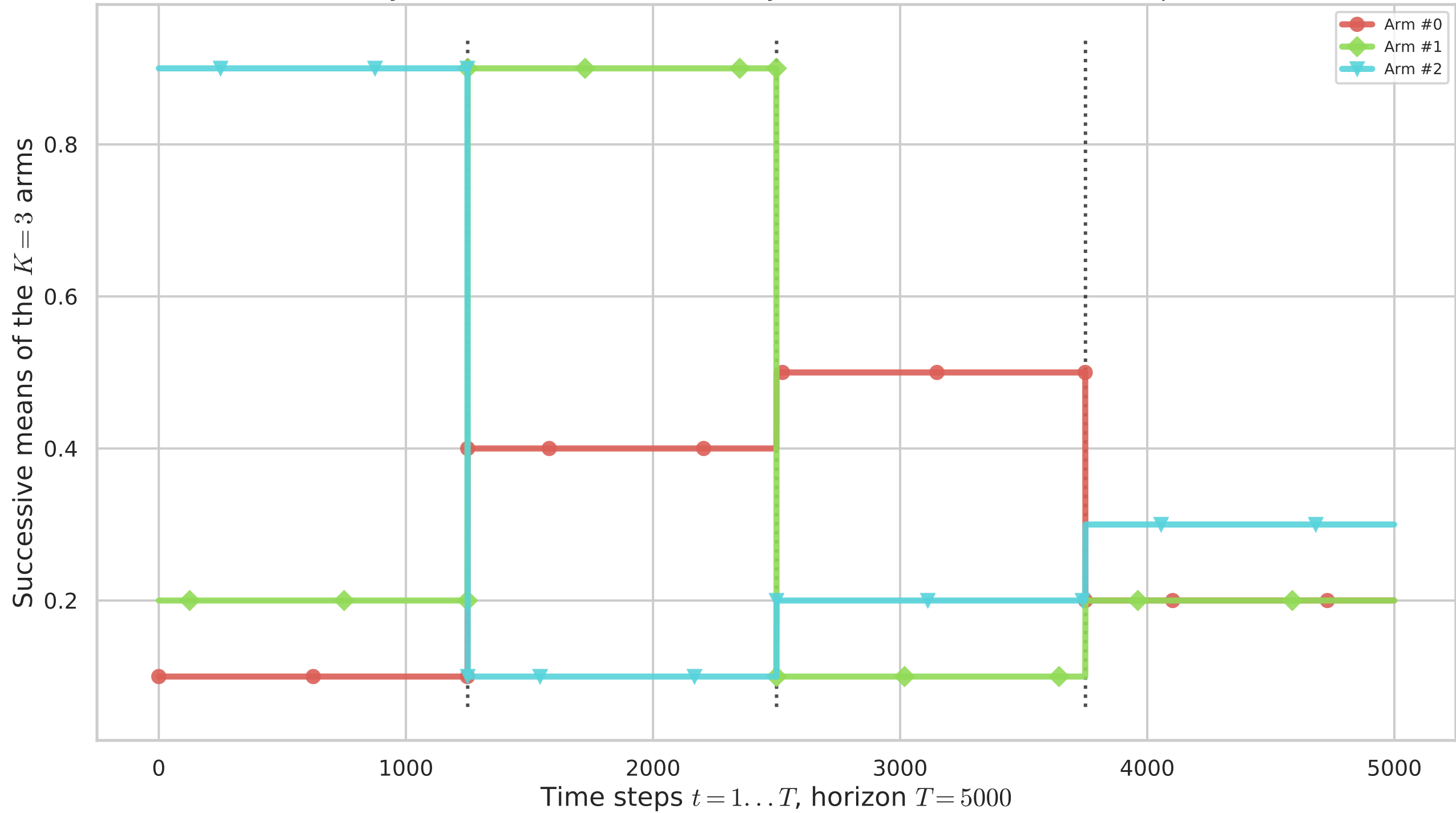
History of means for Non-Stationary MAB, Bernoulli with 3 break-points
