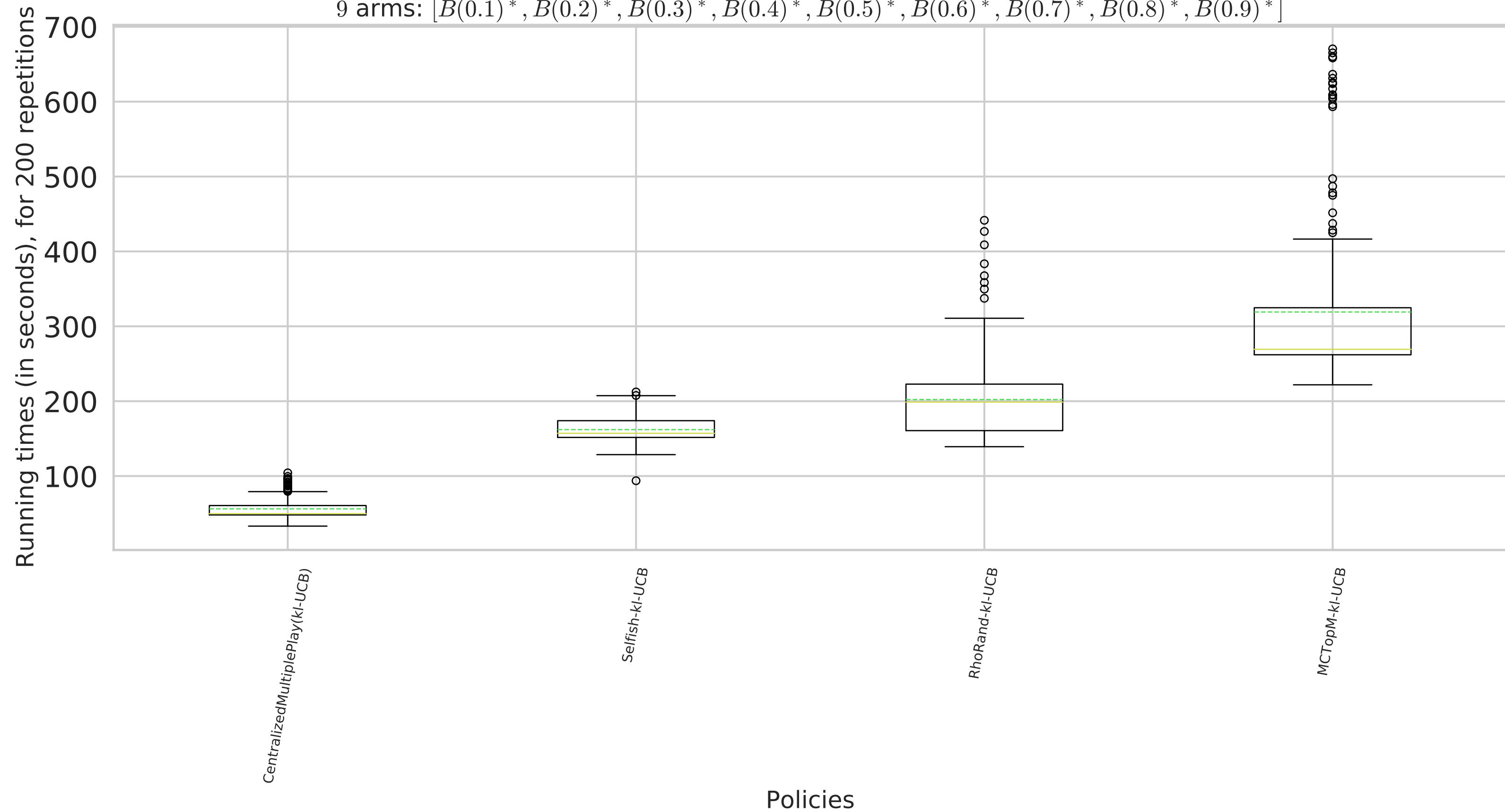
Running times for different MP bandit algorithms, horizon T=10000 , averaged 200 times
