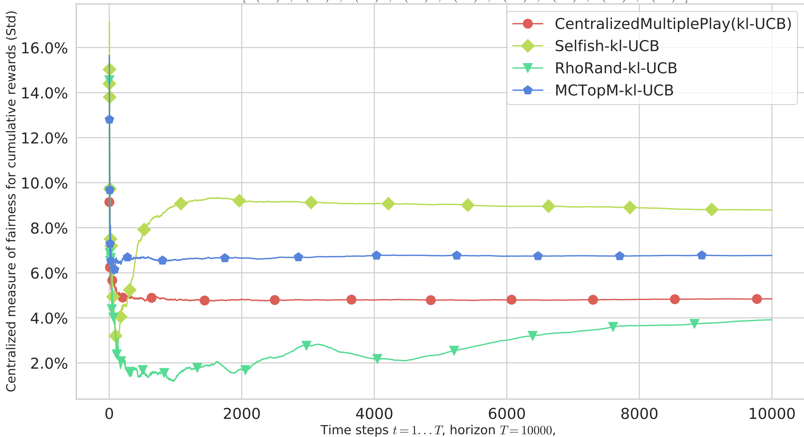
Multi-players M=9 : Centralized measure of fairness, averaged 200 times 9 arms: [B(0.1)^*, B(0.2)^*, B(0.3)^*, B(0.4)^*, B(0.5)^*, B(0.6)^*, B(0.7)^*, B(0.8)^*, B(0.9)^*]
