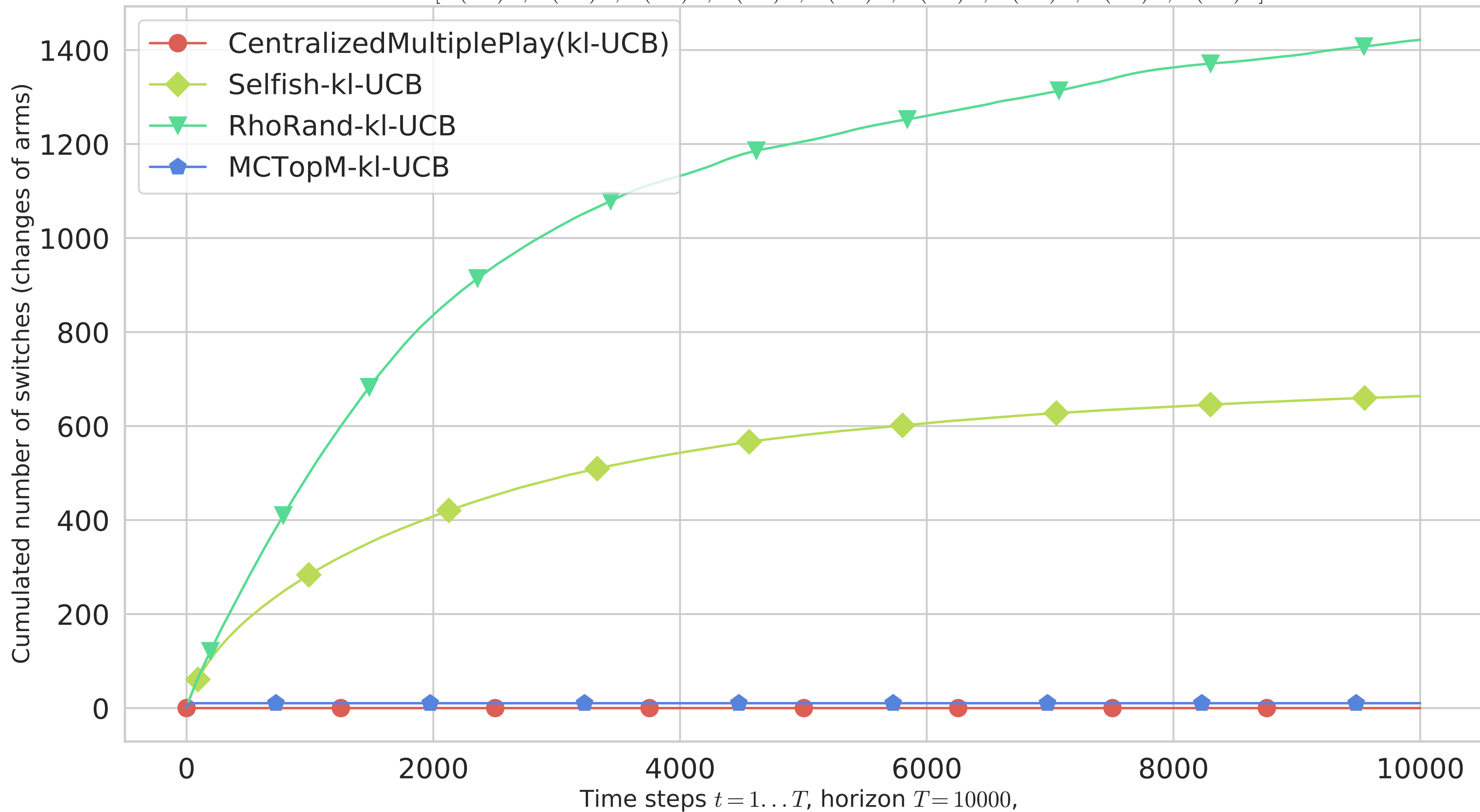
Multi-players M=9 : Total cumulated number of switches, averaged 200 times 9 arms: [B(0.1)^*, B(0.2)^*, B(0.3)^*, B(0.4)^*, B(0.5)^*, B(0.6)^*, B(0.7)^*, B(0.8)^*, B(0.9)^*]
