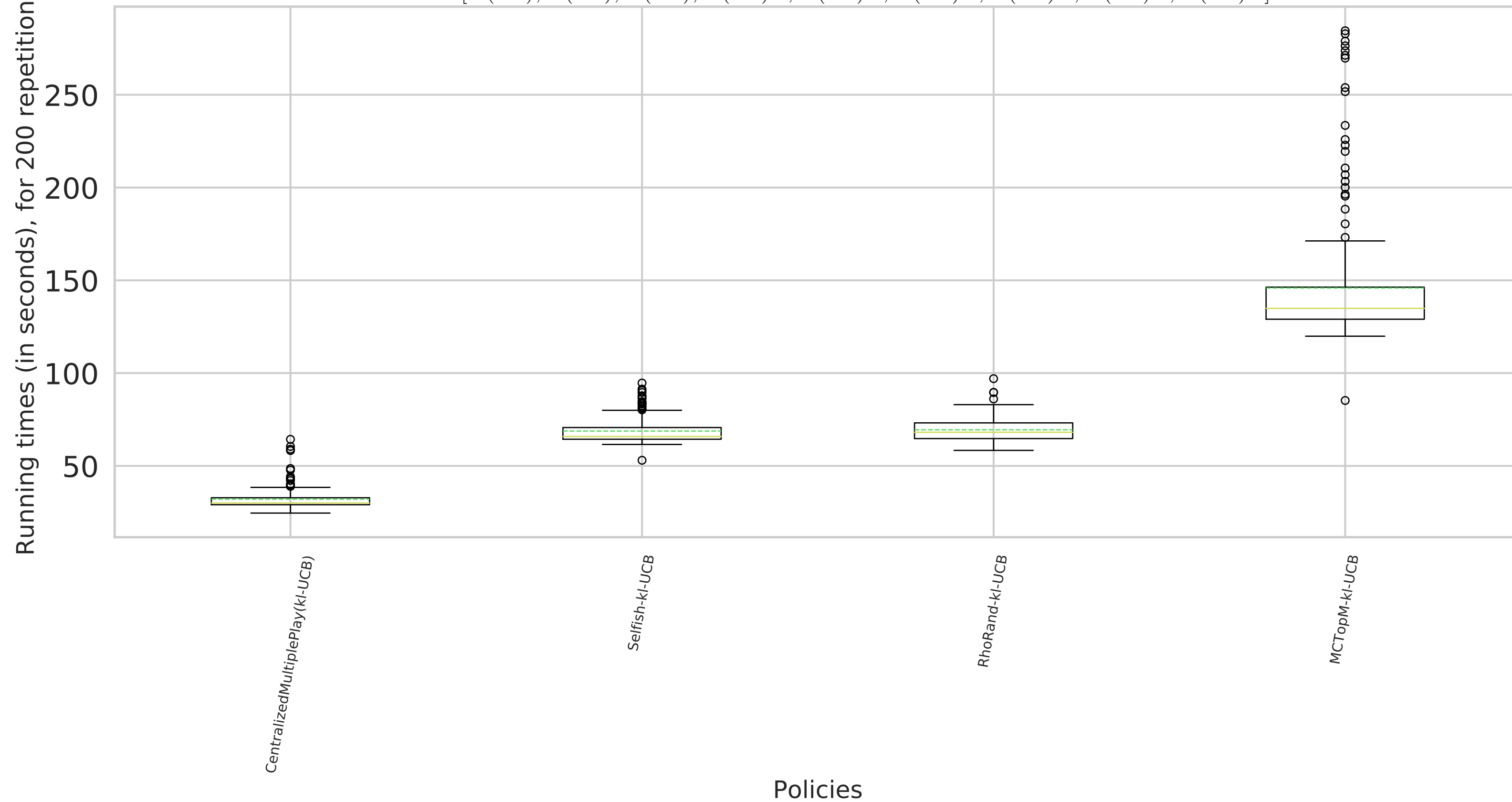
Running times for different MP bandit algorithms, horizon T=10000 , averaged 200 times 9 arms: [B(0.1), B(0.2), B(0.3), B(0.4)^*, B(0.5)^*, B(0.6)^*, B(0.7)^*, B(0.8)^*, B(0.9)^*]
