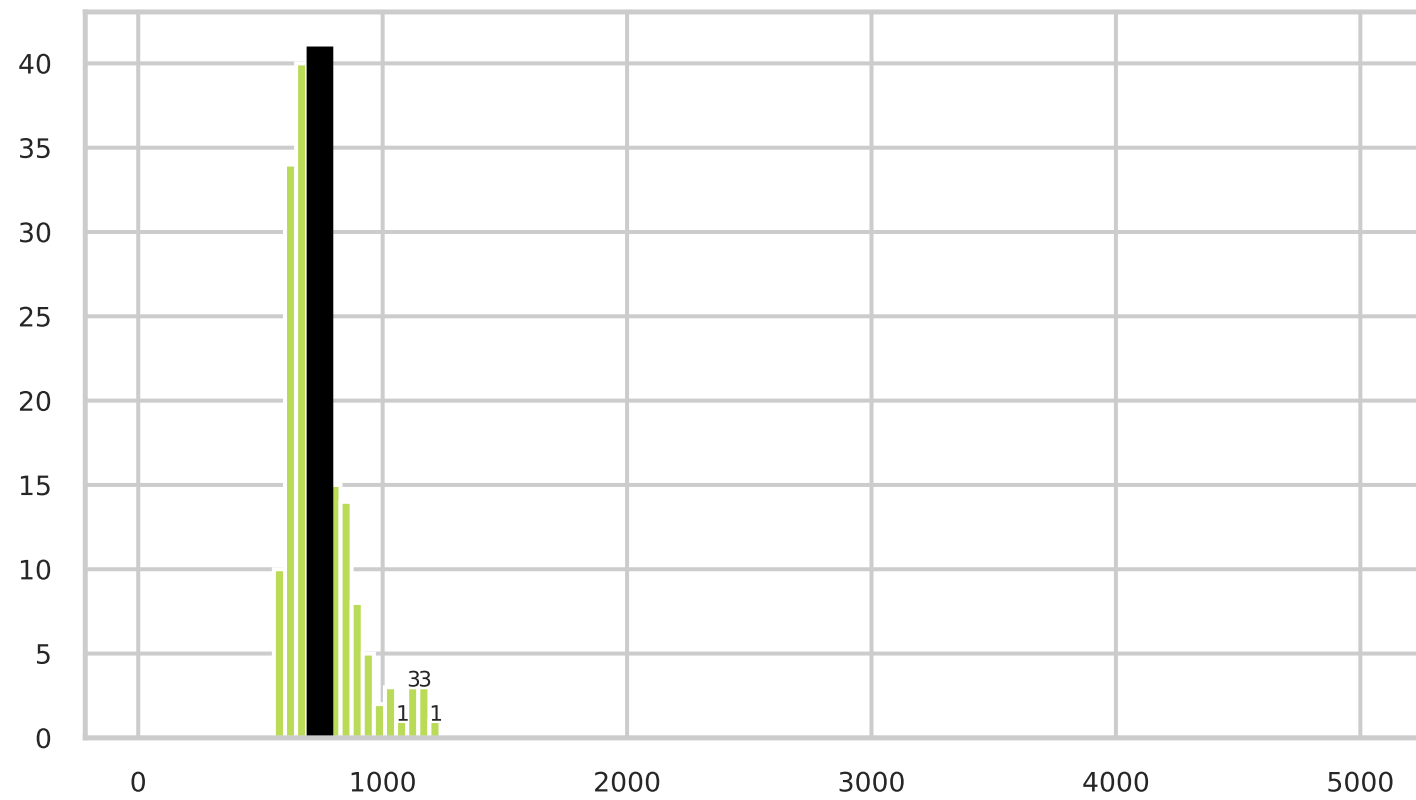
Selfish-kl-UCB
