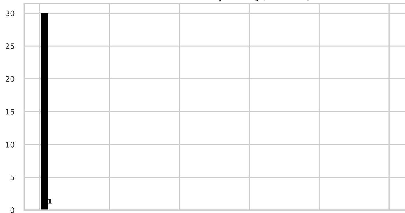
CentralizedMultiplePlay(kl-UCB)
