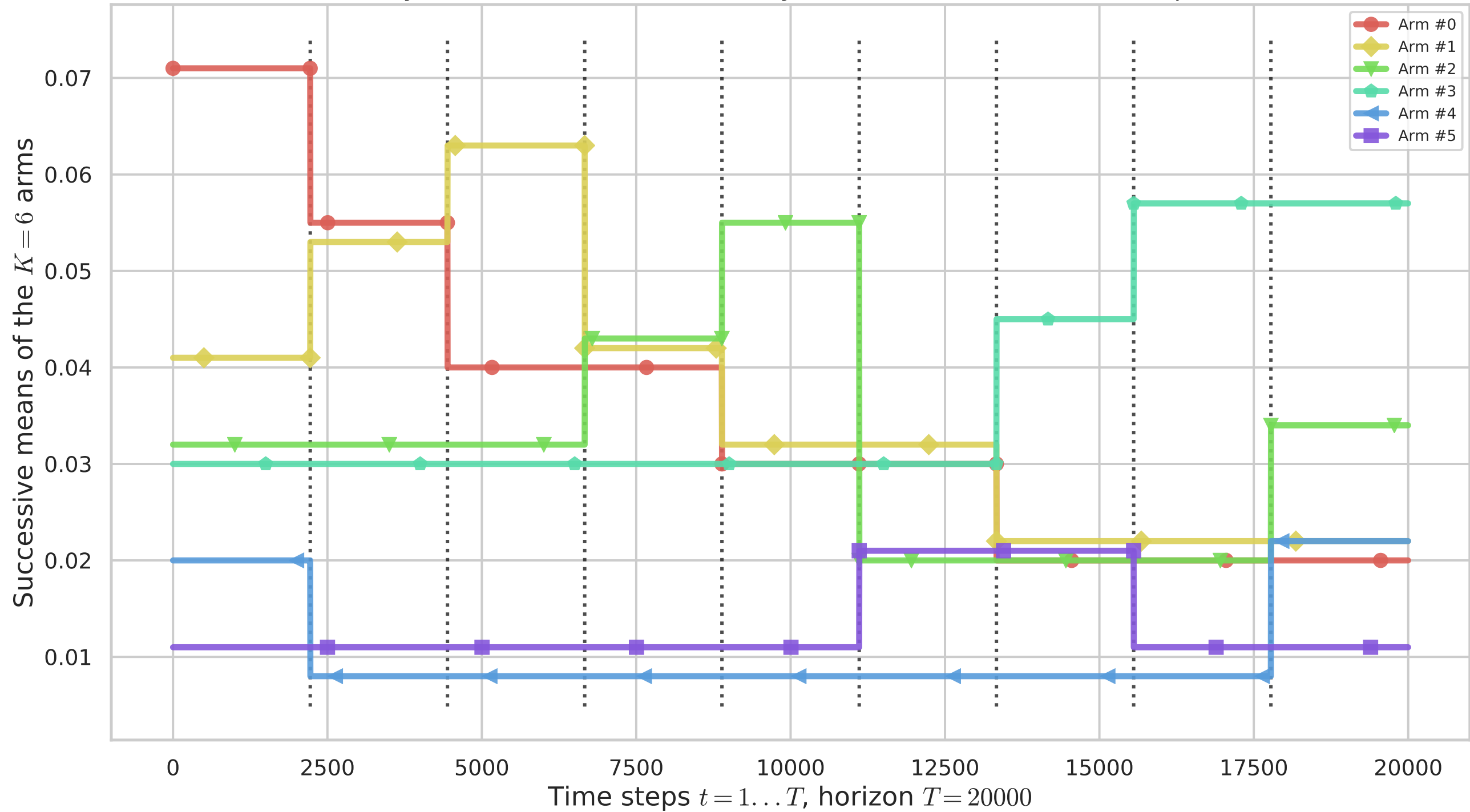
History of means for Non-Stationary MAB, Bernoulli with 8 break-points
