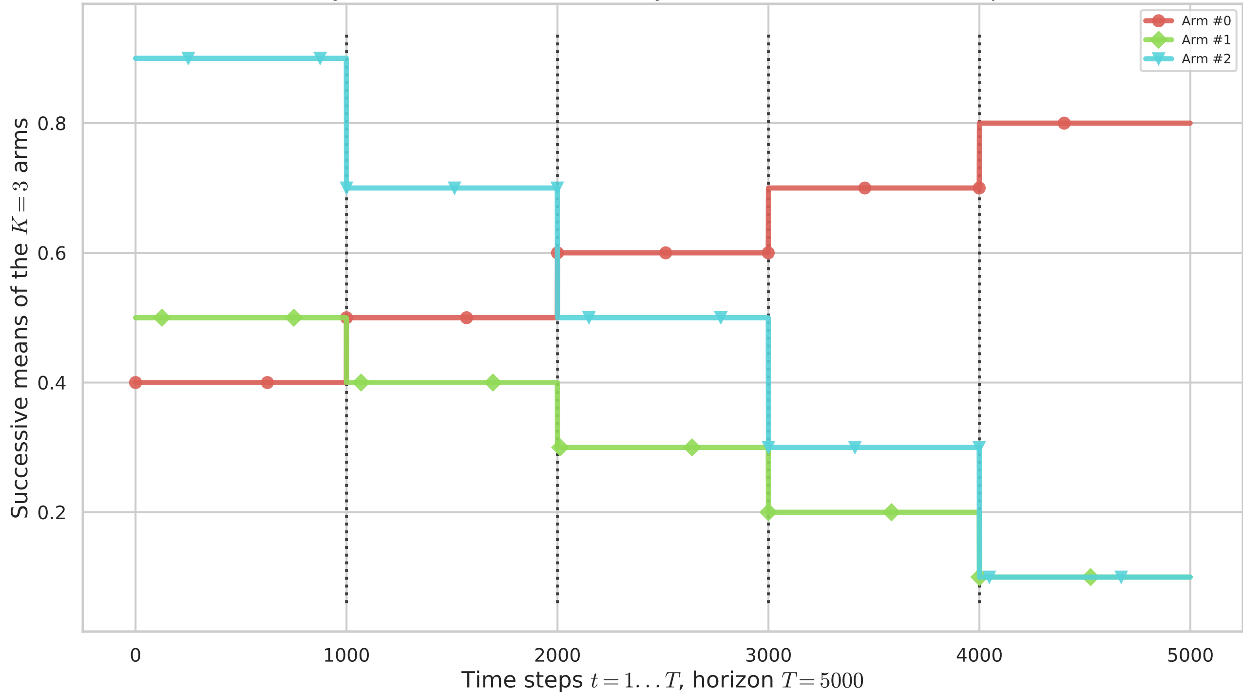
History of means for Non-Stationary MAB, Bernoulli with 4 break-points
