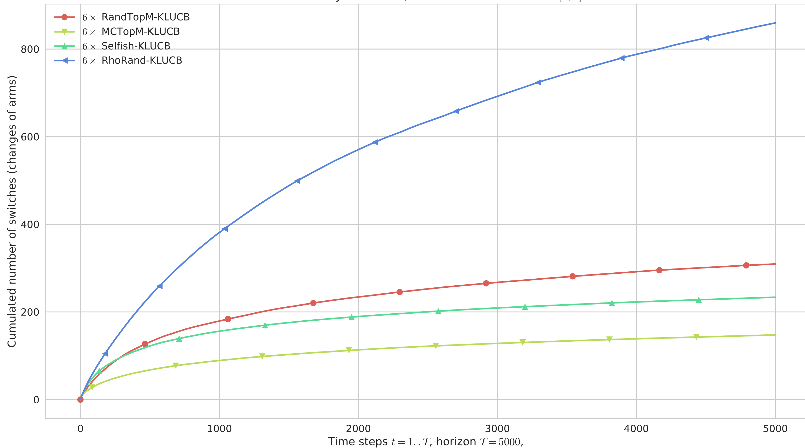
Multi-players M=6 : Total cumulated number of switches, averaged 500 times 9 arms: Bayesian MAB, Bernoulli with means on [0, 1]
