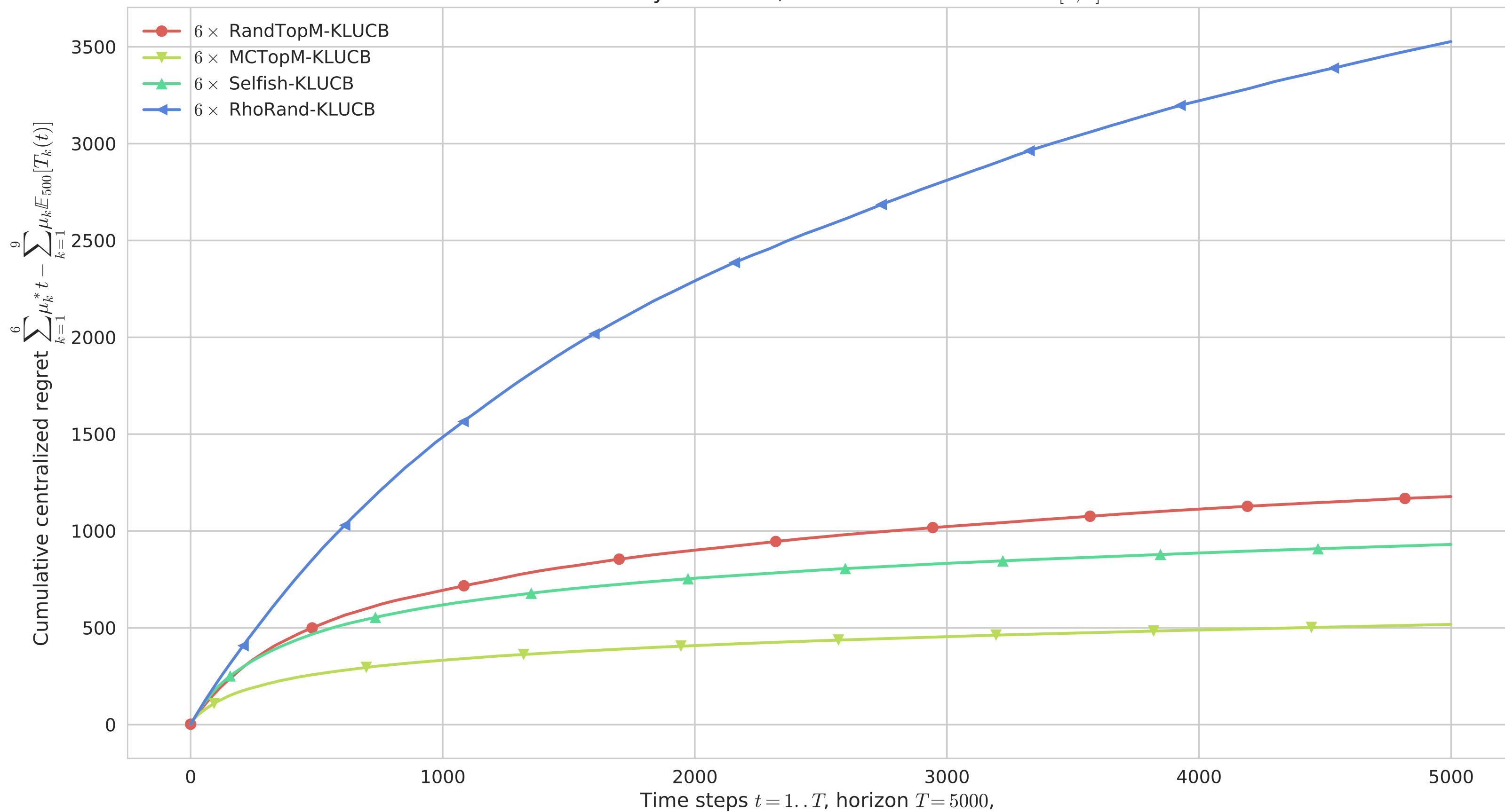
Multi-players M=6 : Cumulated centralized regret, averaged 500 times 9 arms: Bayesian MAB, Bernoulli with means on [0, 1]
