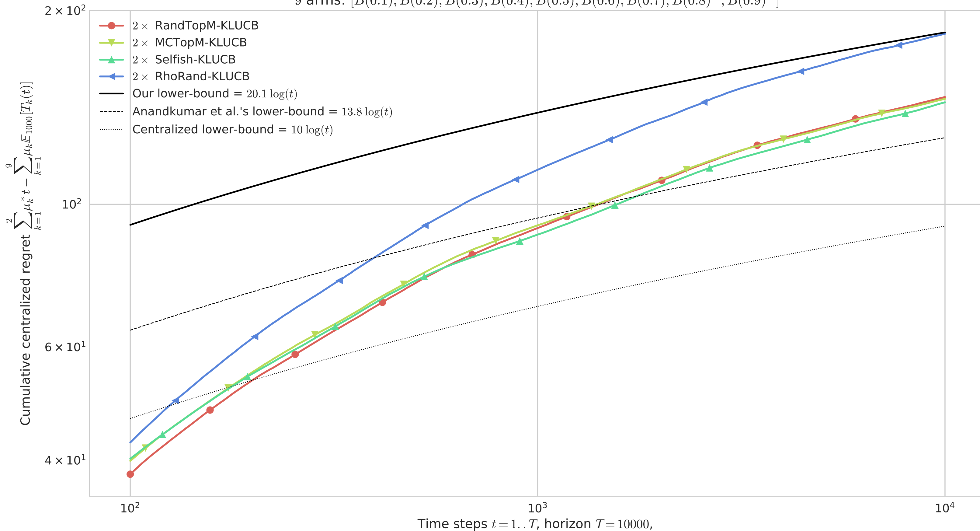
Multi-players M=2 : Cumulated centralized regret, averaged 1000 times 9 arms: [B(0.1), B(0.2), B(0.3), B(0.4), B(0.5), B(0.6), B(0.7), B(0.8)^*, B(0.9)^*]
