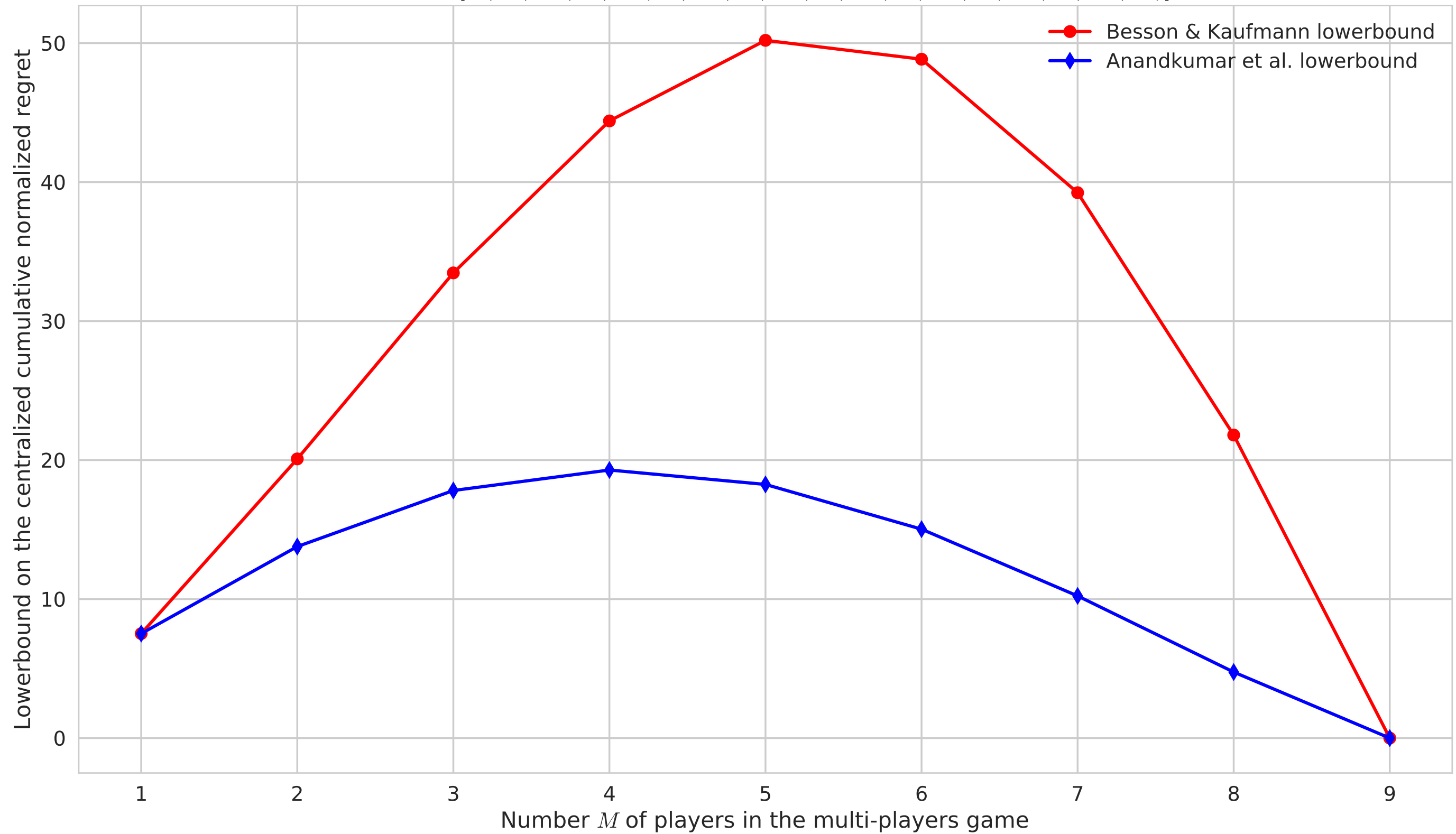
Comparison of our lowerbound and the one from [Anandkumar et al., 2010]. 9 arms: [B(0.1), B(0.2), B(0.3), B(0.4), B(0.5), B(0.6), B(0.7), B(0.8), B(0.9)]
