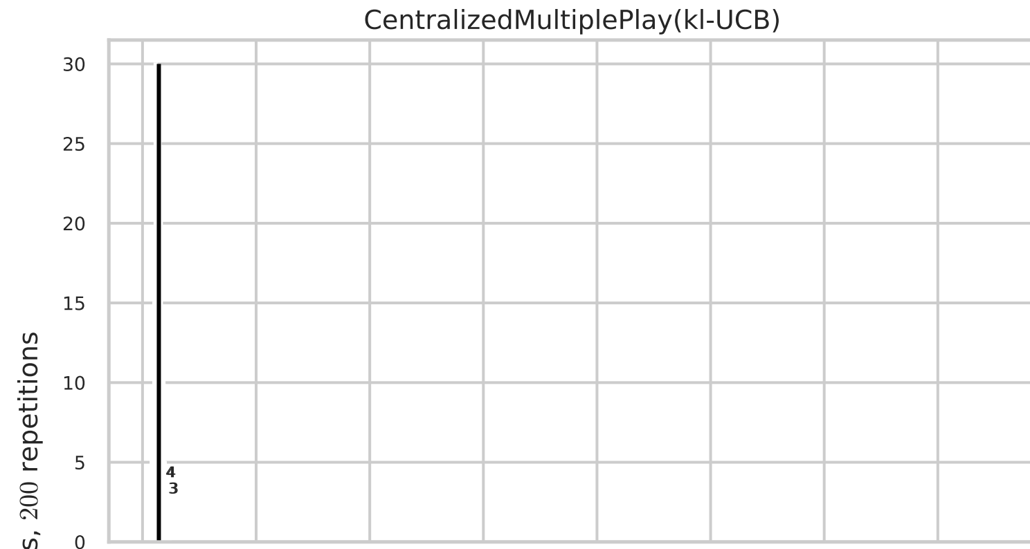
Histogram of regrets for different multi-players bandit algorithms 9 arms: [B(0.1), B(0.2), B(0.3), B(0.4)^*, B(0.5)^*, B(0.6)^*, B(0.7)^*, B(0.8)^*, B(0.9)^*]
