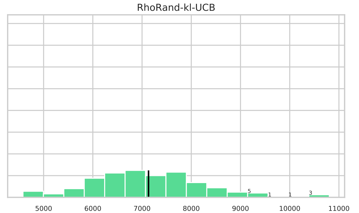
Histogram of regrets for different multi-players bandit algorithms 9 arms: [B(0.1)^*, B(0.2)^*, B(0.3)^*, B(0.4)^*, B(0.5)^*, B(0.6)^*, B(0.7)^*, B(0.8)^*, B(0.9)^*]
