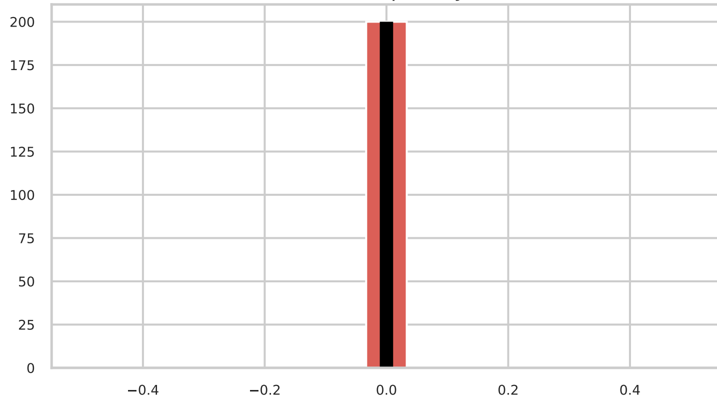
Selfish-kl-UCB
