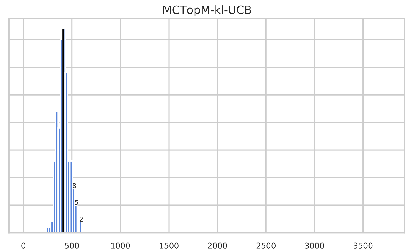
Regret value R_T at the end of simulation, for T=10000
