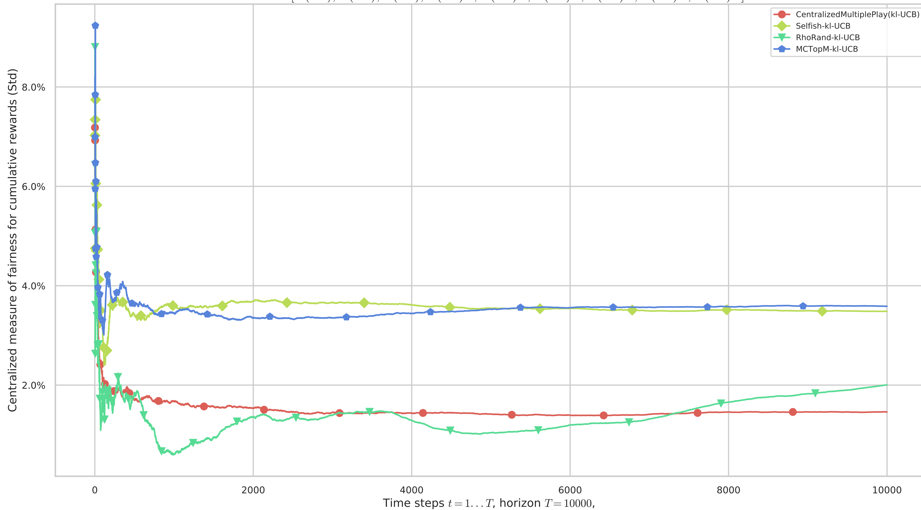
Multi-players M=6 : Centralized measure of fairness, averaged 200 times 9 arms: [B(0.1), B(0.2), B(0.3), B(0.4)^*, B(0.5)^*, B(0.6)^*, B(0.7)^*, B(0.8)^*, B(0.9)^*]
