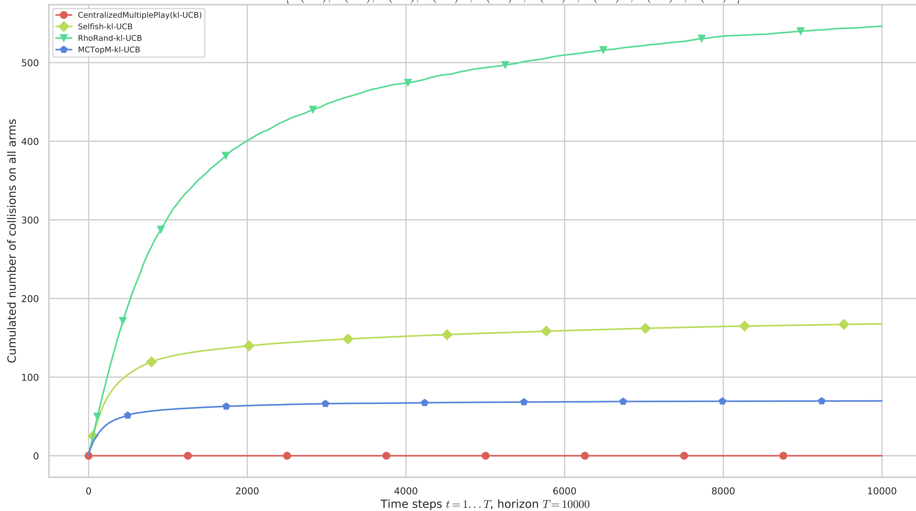
Multi-players M=6 : Cumulated number of collisions, averaged 200 times 9 arms: [B(0.1), B(0.2), B(0.3), B(0.4)^*, B(0.5)^*, B(0.6)^*, B(0.7)^*, B(0.8)^*, B(0.9)^*]
