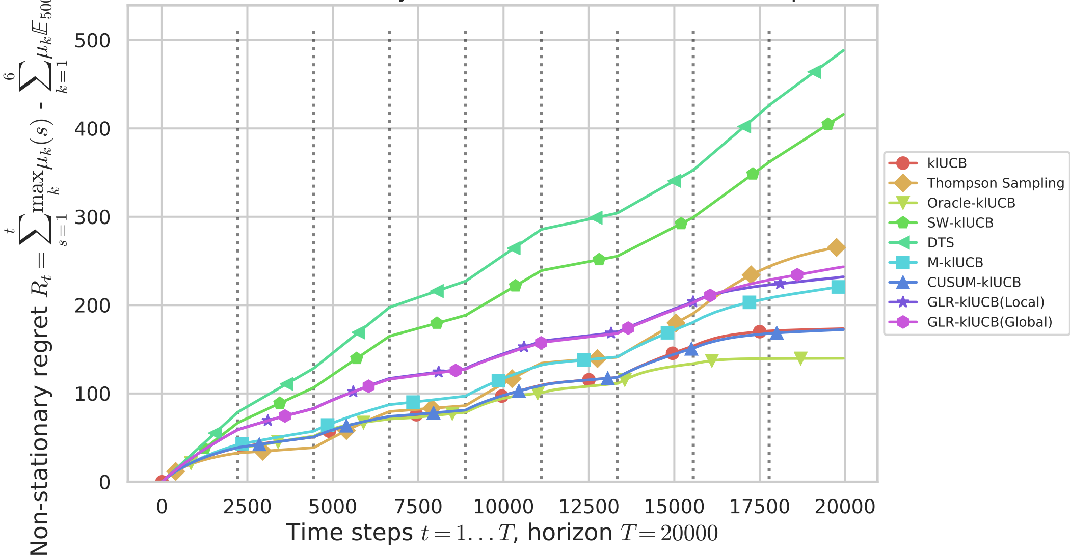
Cumulated regrets for different bandit algorithms, averaged 500 times 6 arms: Non-Stationary MAB, Bernoulli with \Upsilon = 8 break-points
