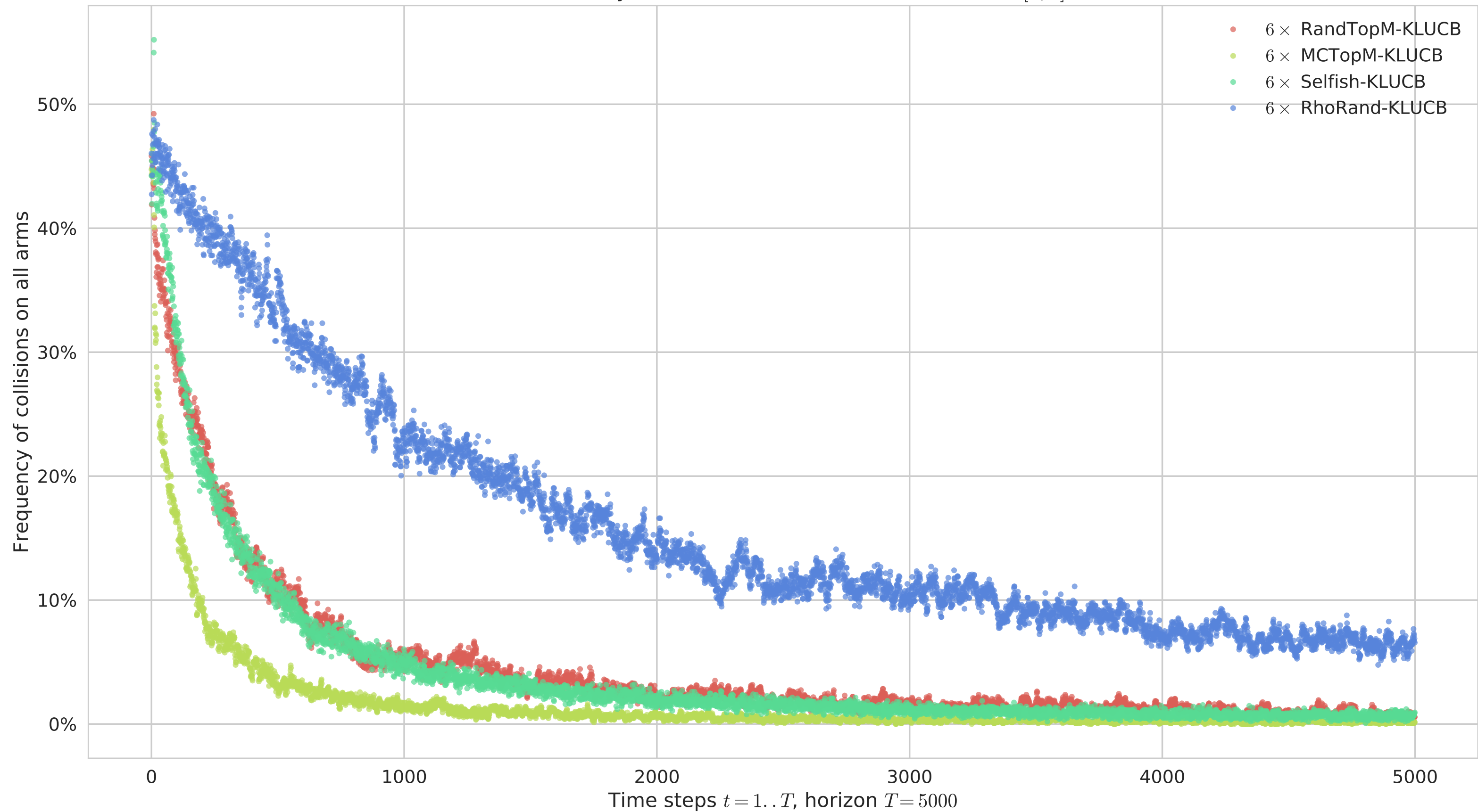
Multi-players M=6 : Frequency of collisions, averaged 500 times 9 arms: Bayesian MAB, Bernoulli with means on [0, 1]
