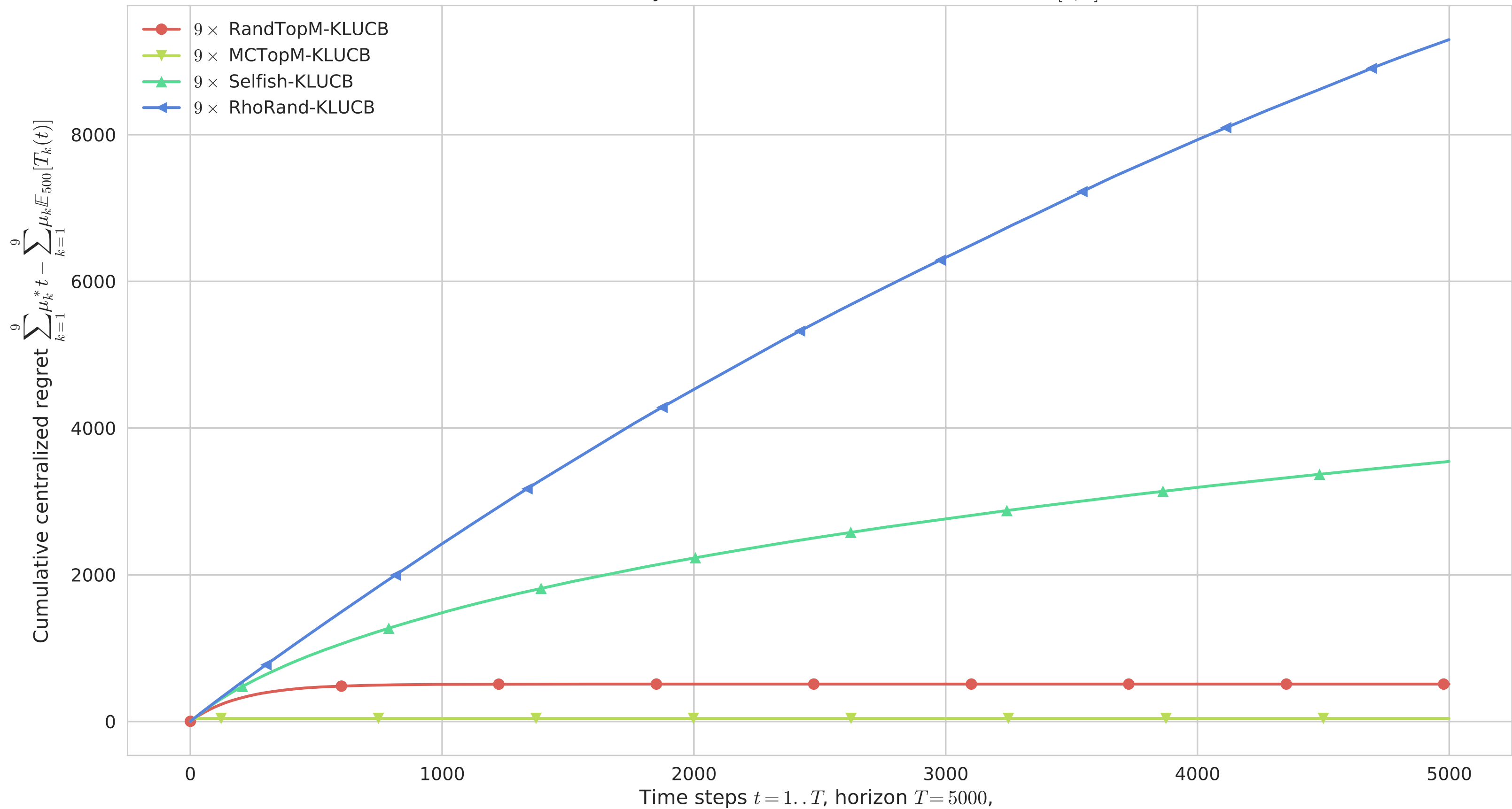
Multi-players M=9 : Cumulated centralized regret, averaged 500 times 9 arms: Bayesian MAB, Bernoulli with means on [0, 1]
