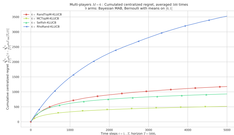
Figure 1: Regret, M = 6 players, K = 9 arms, horizon T = 5000 , against 500 problems \boldsymbol{\mu} uniformly sampled in [0, 1]^K . RhoRand (top blue curve) is outperformed by the other algorithms (and the gain increases with M ). MCTopM (bottom yellow) outperforms all the other algorithms in most cases.
