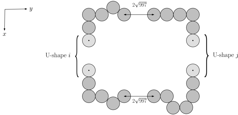
Figure 5: A U-shape. The distance constraint the spine balls to use inflation vectors orthogonal to those of the U-shape.
