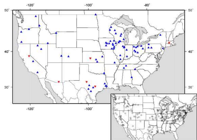
Figure 2. Annual trends in streamflow observed from the HCD Network. Upward (blue triangles) and downward (red inverted triangles) trends are shown in the larger map. The smaller map shows the spatial coverage of the HCDN stations.
