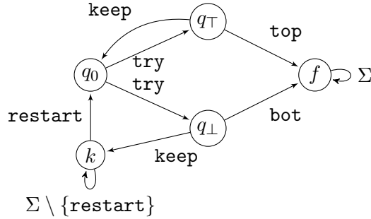
Figure 2: A second example of NFA for the population control problem: \mathcal{A}_{\text{time}} .
