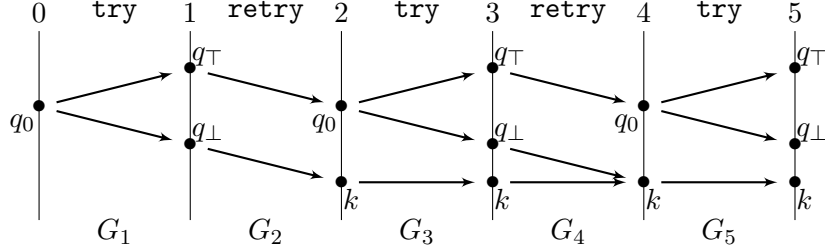
Figure 7: Sequence of graphs associated with a run.
