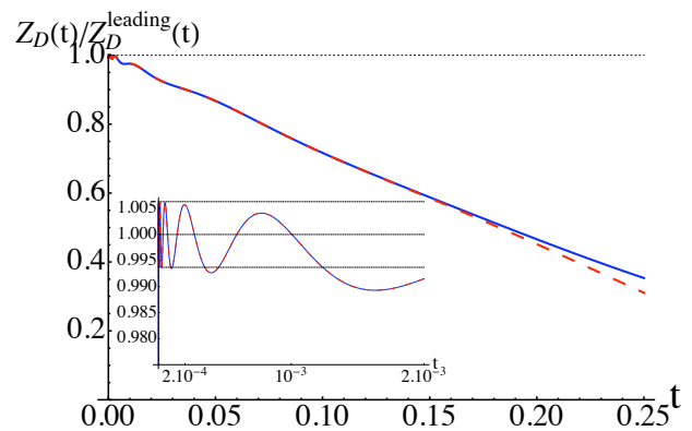
FIG. 3: Heat kernel Z_D(t) at small time, normalized by the leading non-oscillating term, for the fractal diamond D_{4,2} . The solid [blue] curve is exact; the dashed [red] curve is the approximate expression (9). At very small t , these curves are indistinguishable, as shown in the inset plot. The relative amplitude of the oscillations remains constant as t \rightarrow 0 .
