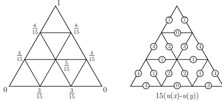
FIGURE 6. The harmonic extension of u on SG_3 , where u|_{V_0} = [1, 0, 0] .
