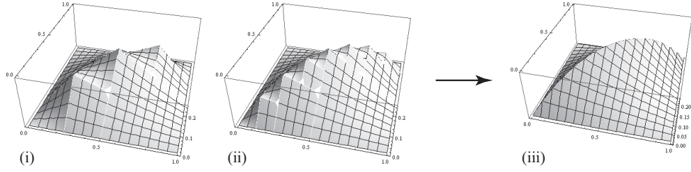
FIGURE 2. Mathematica plot of G^{(\lambda)} for \lambda = 1 and two of its partial sums. (i) The sum of (a) and (b) in Fig. 1. (ii) The sum of (a), (b), (c) in Fig. 1. (iii) The resolvent kernel G^{(\lambda)}(x, y) obtained in the limit.
