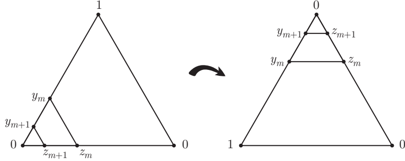
FIGURE 8. The values of the eigenfunction u on SG_3 , where u|_{V_0} = [0, 1, 0]^T . This figure shows a closeup of u near a point where it takes the value 0. We define y_m := u(F_1^m q_0) and z_m := u(F_1^m q_2) .
