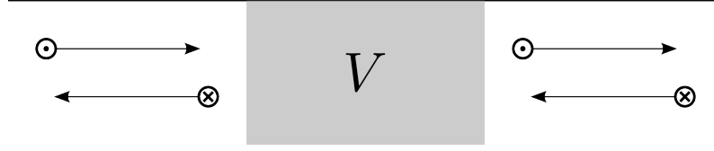
Fig. 8.4 Scattering of an edge state on a time-reversal symmetric defect V . In a two-dimensional time-reversal invariant topological insulator with a single Kramers pair of edge states, the incoming electron is transmitted through such a defect region with unit probability.
