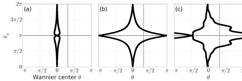
Fig. 9.1 Wilson loop examples.
