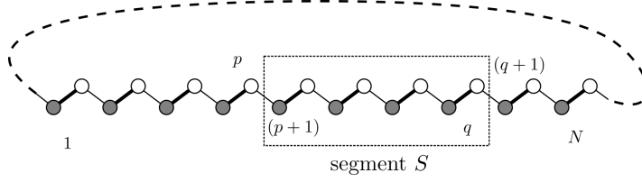
Fig. 5.1 A segment enclosed by two cross sections in the one-dimensional SSH model. The segment S is defined as the part of the chain between the p th and (q+1) th unit cells. The current operators corresponding to the two cross sections can be established by considering the temporal change of the number of particles in the segment. The dashed line represents the periodic boundary condition.
