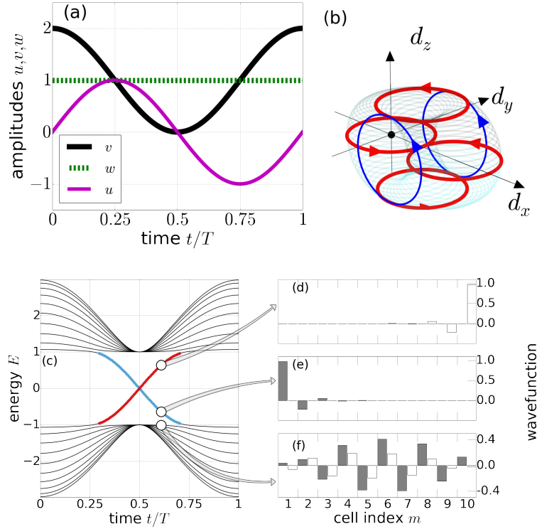
Fig. 4.3 The smooth pump sequence of the Rice-Mele model for \bar{\nu} = 1 . The hopping amplitudes and the sublattice potential (a) are varied smoothly as a function of time. The vector \mathbf{d}(k,t) corresponding to the bulk momentum-space Hamiltonian (b) traces out a torus in the 3-dimensional space. Instantaneous spectrum of the Hamiltonian \hat{H}(t) on an open chain of N = 10 sites (c) reveals that during a cycle, one state crosses over to the upper band on the right edge, and one to the lower band on the left edge (dark red/light blue highlights energies of edge states, whose wavefunctions have than 60% weight on the rightmost/leftmost 2 unit cells). The wavefunctions of the edge states (d,e) are exponentially localized to one edge and have support overwhelmingly on one sublattice each. In contrast a typical bulk state (f) has a delocalized wavefunction with support on both sublattices. .
