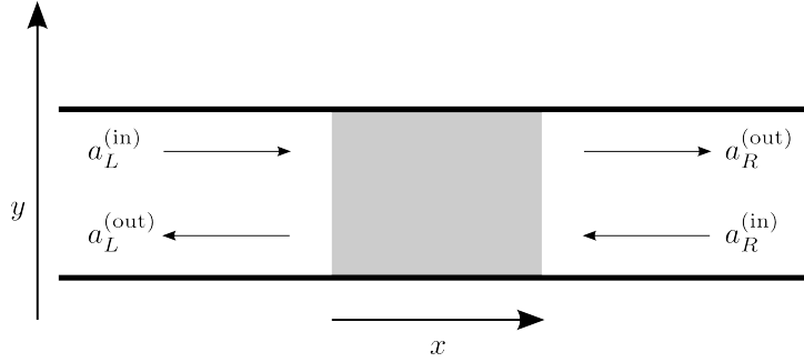
Fig. 8.3 Disordered region (gray) obstructing electrons in a two-dimensional phase-coherent conductor. The scattering matrix S relates the amplitudes a_L^{(in)} and a_R^{(in)} of incoming waves to the amplitudes a_L^{(out)} and a_R^{(out)} of outgoing waves.
