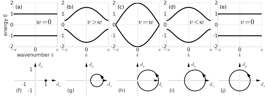
Fig. 1.2 Dispersion relations of the SSH model, Eq. (1.15), for five settings of the hopping amplitudes: (a): v = 1, w = 0 ; (b): v = 1, w = 0.6 ; (c): v = w = 1 ; (d): v = 0.6, w = 1 ; (e): v = 0, w = 1 . In each case, the path of the endpoints of the vector \mathbf{d}(k) representing the bulk momentum-space Hamiltonian, Eqs. (1.17) and (1.18), are also shown on the d_x, d_y plane, as the wavenumber is swept across the Brillouin zone, k = 0 \rightarrow 2\pi .
