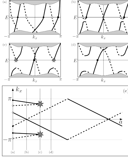
Fig. 8.2 Edge states on a single edge of a 2-dimensional time-reversal invariant topological insulator with \hat{\mathcal{F}}^2 = -1 , as the edge region undergoes a continuous deformation, parametrized by a , respecting the symmetry and the translational invariance along the edge. In (a)–(d), the edge state dispersions relations are shown, in the full edge Brillouin zone k_x = -\pi, \dots, \pi , and in the energy window corresponding to the bulk gap. For clarity, right- (left-) propagating edge states are denoted by continuous (dashed) lines. Due to the deformation of the Hamiltonian, the edge state branches can move, bend, and couple, while the bulk remains unchanged. From (a) to (b), the crossing points between counterpropagating edge states become anticrossings, i.e., gaps open in these pairs of dispersion relation branches as a usual consequence of any parameter coupling them. Crossings at k_x = 0 and k_x = \pi cannot be gapped, as this would lead to a violation of the Kramers theorem. From (b) to (d), these gaps become so large that at energy E = 0 , the number of edge states drops from 6 (3 Kramers pairs) to 2 (1 Kramers pair). The k_x values of the edge states at 0 energy are plotted in (e), where this change in the number of edge states shows up as an “annihilation” of right-propagating and left-propagating edge states.
