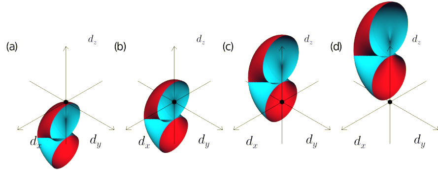
Fig. 6.3 The torus \mathbf{d}(\mathbf{k}) of the QWZ model for different values of u keeping A = 1 . For clarity only the image of half of the Brillouin zone is shown. In (a) and (d) u = \mp 2.2 and the torus does not contain the origin hence Q = 0 . In (b) u = -1 , taking an infinite line from the origin along the positive z axis we hit the blue side of the torus once hence Q = -1 . In (c) u = 1 , taking the infinite line in the negative z direction we hit the red side of the torus thus Q = 1 .
