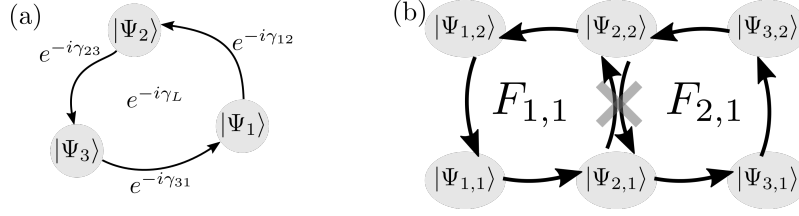
Fig. 2.1 Berry phase, Berry flux and Berry curvature for discrete quantum states. (a) The Berry phase \gamma_L for the loop L consisting of N = 3 states is defined from the relative phases \gamma_{12} , \gamma_{23} , \gamma_{31} . (b) The Berry phase of a loop defined on a lattice of states can be expressed as the sum of the Berry phases F_{1,1} and F_{2,1} of the plaquettes enclosed by the loop. The plaquette Berry phase F_{n,m} is also called Berry flux.
