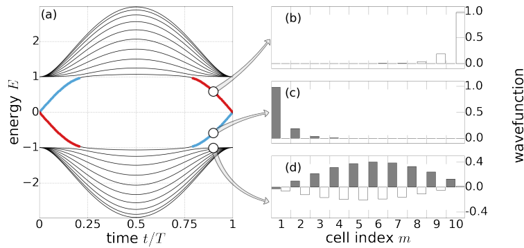
Fig. 4.6 The smooth pump sequence of the Rice-Mele model for \bar{v} = -1 , revealing reversed pumping with respect to the \bar{v} = 1 case. (a) Instantaneous spectrum of the Hamiltonian \hat{H}(t) on an open chain of N = 10 sites. During a cycle, one edge state on the left (light blue) crosses over from the valence to the conduction band, revealing that there is a single particle per cycle is pumped from right to left in the valence band. Wavefunctions of the edge states (b,c) as well as a typical bulk state (d) are also shown.
