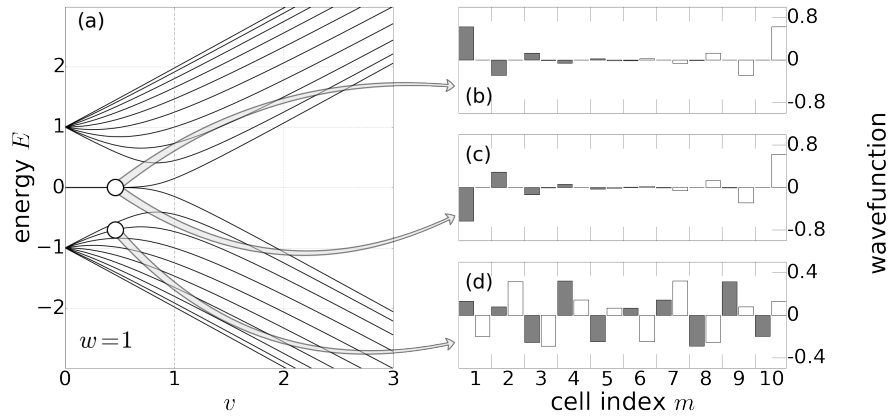
Fig. 1.4 Energy spectrum and wave functions of a finite-sized SSH model. The number of unit cells is N = 10 . (a) Energy spectrum of the system for intercell hopping amplitude w = 1 as a function of the intracell hopping amplitude v . v < 1 ( v > 1 ) corresponds to the topological (trivial) phases. (b) and (c) show the wave functions of the hybridized edge states, while (d) shows a generic bulk wave function.
