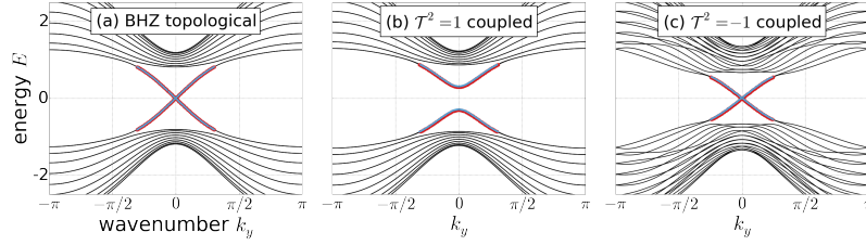
Fig. 8.1 Stripe dispersion relations of the BHZ model, with sublattice potential parameter u = -1.2 . Right/left edge states (more than 60% weight on the last/first two columns of unit cells) marked in dark red/light blue. (a): uncoupled layers, \hat{C} = 0 . (b): Symmetric coupling \hat{C} = 0.3\sigma_x gaps the edge states out. (c): Antisymmetric coupling \hat{C} = 0.3\sigma_y cannot open a gap in the edge spectrum.
