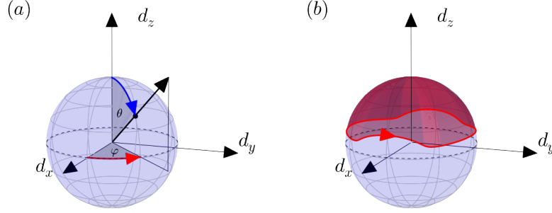
Fig. 2.2 The Bloch sphere. A generic traceless gapped two-level Hamiltonian is a linear combination of Pauli matrices, \hat{H}(\mathbf{d}) = \mathbf{d} \cdot \hat{\sigma} . This can be identified with a point in \mathbb{R}^3 \setminus \{0\} . The eigenenergies are given by the distance of the point from the origin, the eigenstates depend only on the direction of the vector \mathbf{d} , i.e., on the angles \theta and \varphi , as defined in subfigure (a) and in Eq. (2.62). The Berry phase of a closed curve \mathcal{C} is half the area enclosed by the curve when it is projected onto the surface of the Bloch sphere.
