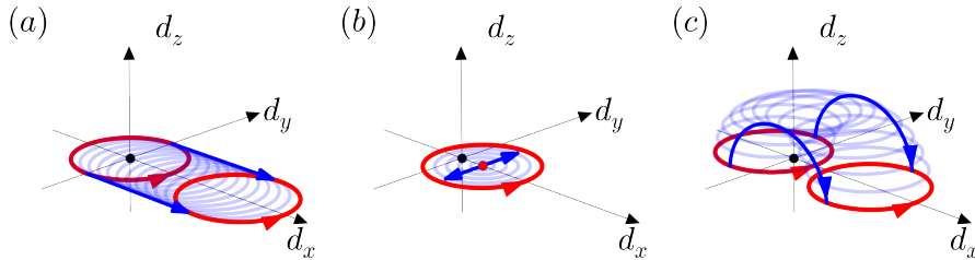
Fig. 1.6 The endpoints of the vector \mathbf{d}(k) as k goes across the Brillouin zone (red or blue closed circles), for various parameter settings in the SSH model. In (a), intracell hopping v is set to 0.5, and intercell hopping is gradually increased from 0 to 1 (outermost red circle). In the process, the bulk gap was closed and reopened, as the origin (black point) is included in some of the blue circles. The winding number changed from 0 to 1. In (b), we gradually decrease intracell hopping v to 0 so that the winding number again changes to 1. In the process, the bulk gap closes and reopens. In (c), keeping w = 1 , we increase the intracell hopping from 0.5 to 2.5, but avoid closing the bulk gap by introducing a sublattice potential, H_{\text{sublattice}} = u\hat{\sigma}_z . We do this by tuning a parameter \theta from 0 to \pi , and setting v = 1.5 - \cos \theta , and u = \sin \theta . At the end of the process, \theta = 0 , there is no sublattice potential, so chiral symmetry is restored, but the winding number is 0 again.
