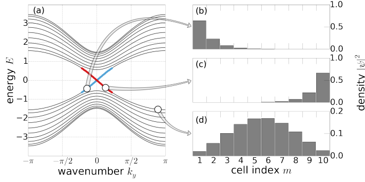
Fig. 6.5 Dispersion relation of a strip of QWZ model, of width N = 10 , and sublattice potential parameter u = -1.5 . Because the strip is translation invariant along the edge, the wavenumber k_y is a good quantum number, and the energy eigenvalues can be plotted (a) as a function of k_y , forming branches of a dispersion relation. Light blue/dark red highlights energies of edge states, whose wavefunction has over 60% weight on unit cells with m_x \leq 2 / m_x \geq N - 1 . These are parts of the N th and N + 1 th branch, which split off from the bulk around -\pi/4 < k_y < \pi/4 , and have an avoided crossing with an exponentially small gap near k_y = 0 . We show the marginal position probability distribution of the N th energy eigenstate, P_N(m_x) = \sum_{\alpha \in \{A,B\}} \sum_{m_y} |\langle m_x, \alpha | \Psi_N \rangle|^2 , for three values of k_y . Depending on k_y , this state can be an edge state on the right edge (b), on the left edge (c), or a bulk state (d).
