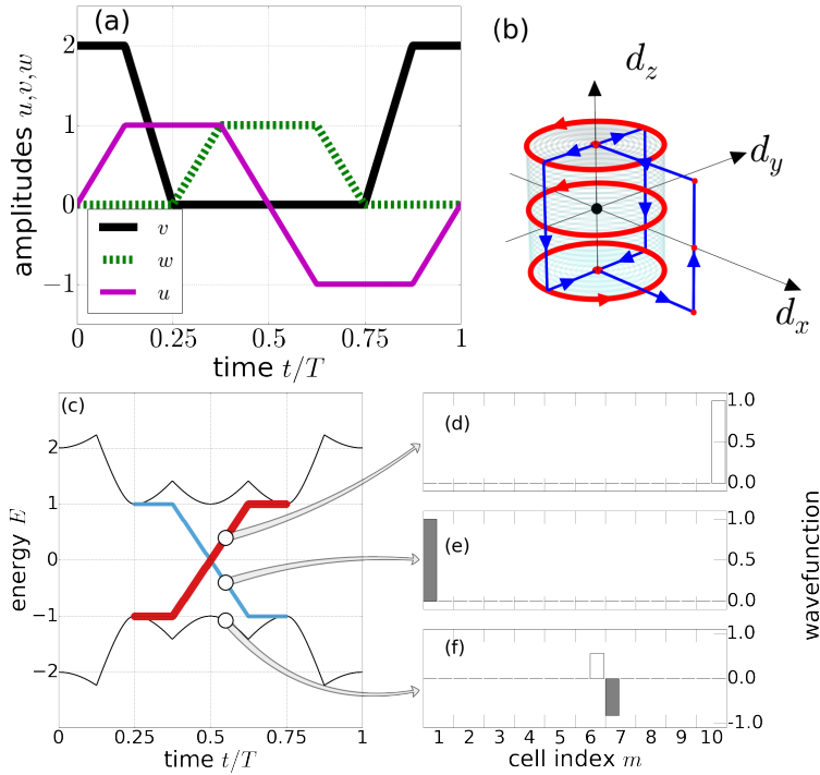
Fig. 4.1 The control freak pump sequence in the Rice-Mele model. The sequence is defined via Eqs. (4.5) and (4.6). (a) Time dependence of the hopping amplitudes v , w and the sublattice potential u . (b) The surface formed by the vector \mathbf{d}(k, t) corresponding to the bulk momentum-space Hamiltonian. The topology of the surface is a torus, but its parts corresponding to t \in [0, 0.25]T and t \in [0.75, 1]T are infinitely thin and appear as a line due to the vanishing value of w in these time intervals. (c) Instantaneous spectrum of the Hamiltonian \hat{H}(t) of an open chain of N = 10 sites. Red (blue) points represent states that are localized in the rightmost (leftmost) unit cells and have energies between -1 and 1. (d), (e), (f) Wavefunction plots for different time intervals.
