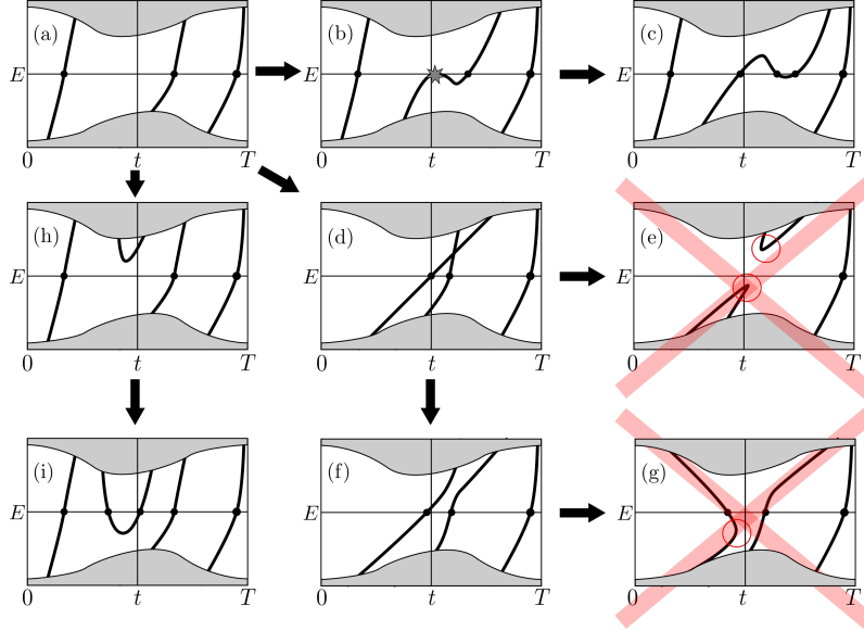
Fig. 4.4 Adiabatic deformations of dispersion relations of edge states on one edge, in an energy window that is deep inside the bulk gap. Starting from a system with 3 copropagating edge states (a), an edge state’s dispersion relation can develop a “bump”, (b)-(c). This can change the number of edge states at a given energy (intersections of the branches with the horizontal line corresponding to the energy), but always by introducing new edge states pairwise, with opposite directions of propagation. Thus the signed sum of edge states remains unchanged. Alternatively, two edge states can develop a crossing, that because of possible coupling between the edge states turns into an avoided crossing (d),(f). This cannot open a gap between branches of the dispersion relation (e), as this would mean that the branches become multivalued functions of the wavenumber k_x (indicating a discontinuity in E(k_x) , which is not possible for a system with short-range hoppings). Therefore, the signed sum of edge states is also unchanged by this process. One might think the signed sum of edge states can change if an edge state’s direction of propagation changes under the adiabatic deformation, as in (g). However, this is also not possible, as it would also make a branch of the dispersion relation multivalued. Deformation of the Hamiltonian can also form a new edge state dispersion branch, as in (a)-(h)-(i), but because of periodic boundary conditions along k_x , this cannot change the signed sum of the number of edge states.
