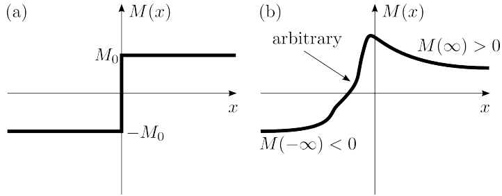
Fig. 7.3 (a) Step-like and (b) irregular spatial dependence of the mass parameter M(x) of the one-dimensional Dirac equation.
