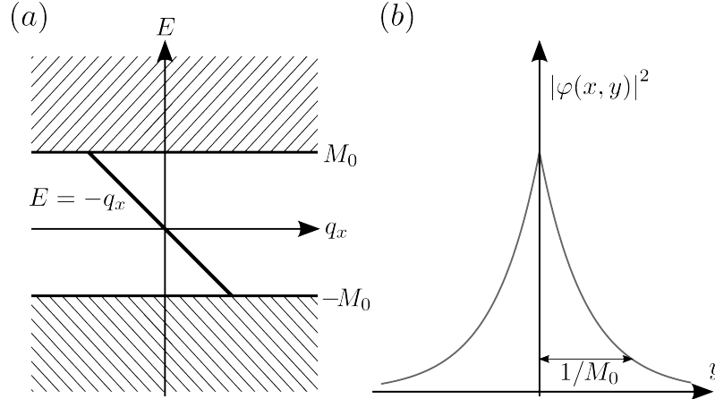
Fig. 7.4 Chiral state obtained from the two-dimensional Dirac equation. (a) Dispersion relation and (b) squared wave function of a chiral state confined to, and propagating along, a mass domain wall.
