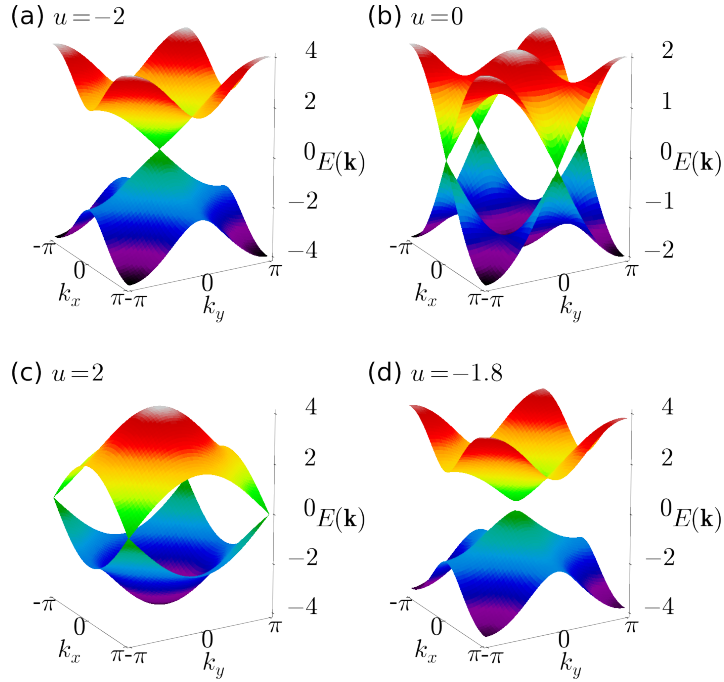
Fig. 6.1 The bulk dispersion relation of the QWZ model, for various values of u , as indicated in the plots. In (a)-(c), the gapless cases are shown, where the bulk gap closes at so-called Dirac points. In (d), a generic value u = -1.8 , the system is insulating.
