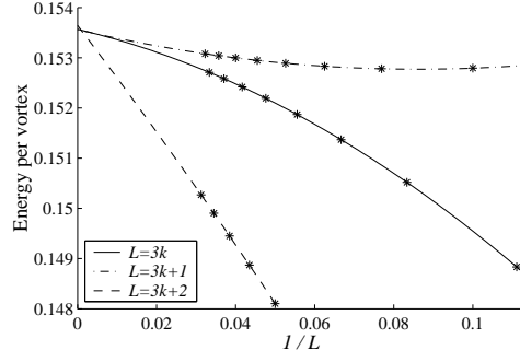
Figure 12: Extrapolation to infinite size: 4 equally spaced vortices on the torus with basis (2Ln_1, 2(Ln_2 + \mathbf{n}_1)) .
