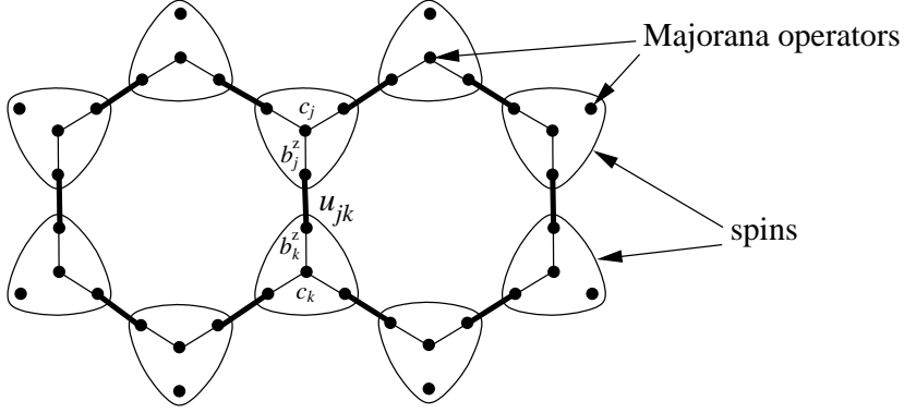
Figure 4: Graphic representation of Hamiltonian (13).
