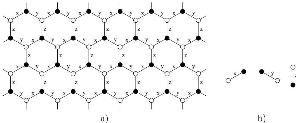
Figure 3: Three types of links in the honeycomb lattice.
