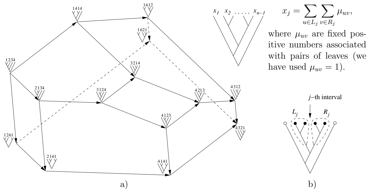
Figure 18: The graph of F -moves between binary planar trees with n = 5 leaves (a) and the procedure used to assign coordinates x_1, \dots, x_{n-1} to each tree (b).
