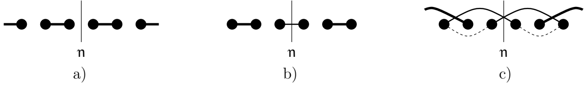
Figure 14: Cutting a Majorana chain: \mathcal{M}_\eta(B) = 1 in cases (a) and (c) whereas \mathcal{M}_\eta(B) = -1 in case (b). The dashed lines in (c) show a possible way to reconnect the broken pairs.
