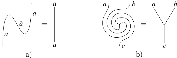
Figure 16: Some “obvious” identities.
