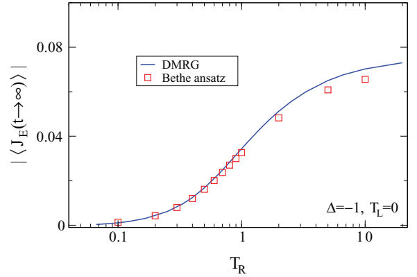
FIG. 8. (Color online) Comparison for the isotropic XXX ferromagnet ( \Delta = -1 ) of two estimates for the function f whose differences give the steady-state energy current J_E via J_E = f(T_L) - f(T_R) between reservoirs T_L and T_R . One estimate is obtained from the DMRG results, using reference temperatures. The other is obtained from the numerical solution of the thermodynamic Bethe ansatz equations and the formula (17).
