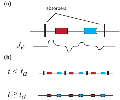
FIG. 7. (Color online) Protocol to prepare a translation-invariant final state with energy current given by the Stefan-Boltzmann prediction. (a) Consider one hot lead and one cold lead, each of which radiates both right and left movers. To create a state that mimics the original two-lead geometry, we place nonunitary “absorbers” as shown. (b) Replicate the geometry of (a) in both directions. The absorbers are maintained in place long enough (until some time t_a ) to absorb half of the excitations from each initial reservoir; which half is absorbed (right or left movers) depends on the reservoir’s temperature. The absorbers are then removed and further evolution is unitary. Energy current is conserved and, if the dispersion of velocities leads to a translation-invariant final state, then the final state must have energy current given by the Stefan-Boltzmann prediction.
