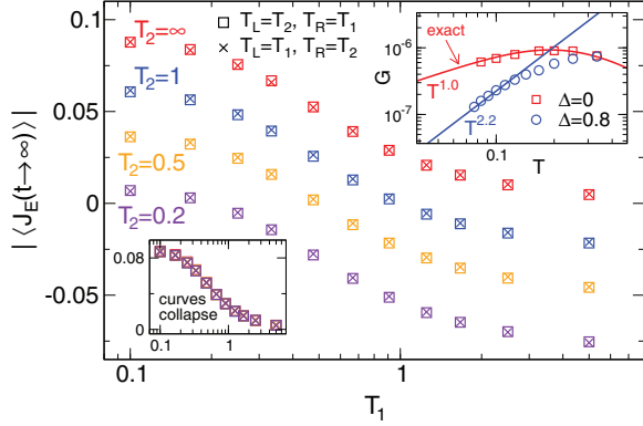
FIG. 9. (Color online) Steady-state current for \lambda = 1 , b = 0 but different bulk interactions \Delta_L = 0.3, \Delta_R = 0.8 and different couplings J_L = 1, J_R = 0.808 to tune the backscattering at the interface to zero. 55 The magnitude of the current is the same for T_L = T_1, T_R = T_2 and T_L = T_2, T_R = T_1 . The curves at different T_2 collapse (left inset), indicating that Eq. (10) still holds. (Right inset) Linear thermal conductance of two identical XXZ chains connected by a strong barrier J_0 = 0.002 . The low- T behavior is consistent with T^{2/K-1} , where K is the Luttinger liquid parameter. 41 At \Delta = 0 we reproduce the exact result of Ref. 35 for any T .
