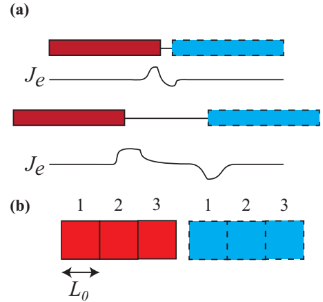
FIG. 6. (Color online) (a) Robustness of total integrated current around a junction: the spatial distribution (drawn schematically for illustrative purposes) of the energy current J_E is different between the geometries with and without a “spacer” region prepared at some reference temperature, but the spatial integrals are the same. (b) Two large reservoirs of size L can be viewed as made up of translated pairs of smaller subreservoirs of size L_0 . The numbers indicate the pairings of the subreservoirs. The sum of many translated copies of a function approaches a constant, as long as the function is smoothly varying on the scale of the translations. If the energy current can indeed be viewed as such a sum, then the existence of a Stefan-Boltzmann function is recovered, independent of the precise shape of the energy current distribution.
