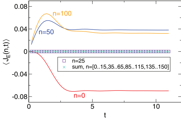
FIG. 5. (Color online) DMRG data for the setup depicted in Fig. 4(b). At t = 0 , three XXZ chains ( \Delta = 0.5 ) of lengths N = 50 and temperatures T_1 = \infty , T_2 = 1 , T_3 = 0.5 are coupled to a ring. The energy currents saturate to their unique steady-state values at the interfaces ( n = 0, 50, 100 ) but remain zero far away from them (e.g., for n = 25 ). The sum of the current over the regions where it is nonzero vanishes [see Eq. (13)] due to the conservation of the total current. As explained in the main text, this motivates the “cyclic sum rule” of Eq. (12), which is equivalent to the existence of a Stefan-Boltzmann function f .
