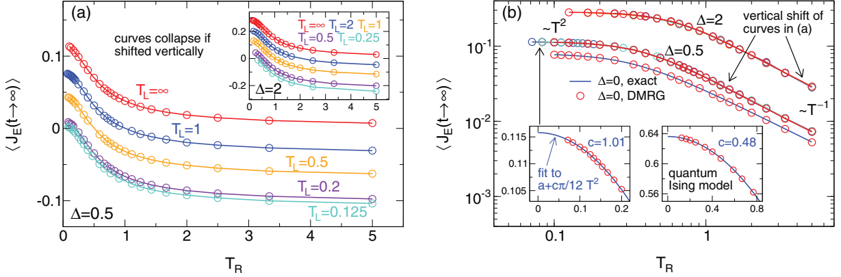
FIG. 3. (Color online) (a) Temperature dependence of the steady-state energy current (which becomes position-independent for t \rightarrow \infty ) of the integrable XXZ chain in the gapless ( \Delta = 0.5 ) and gapped ( \Delta = 2 ) regimes. The right temperature T_R is varied at fixed T_L . (b) The curves at different T_L collapse if shifted vertically; thus the T dependence is of the simple functional form \lim_{t \rightarrow \infty} \langle J_E(n, t) \rangle = f(T_L) - f(T_R) . The linear thermal conductance \sim \partial_T f , therefore, completely determines the nonequilibrium current. A CFT approach 36 predicts universal behavior f(T) = c \frac{\pi}{12} T^2 at low T , which we verify (insets) for the gapless XXZ chain (central charge c = 1 ) and the quantum Ising model ( c = 1/2 ). The free fermion case \Delta = 0 can be solved analytically 34,35 at any T and provides a test for our DMRG numerics.
