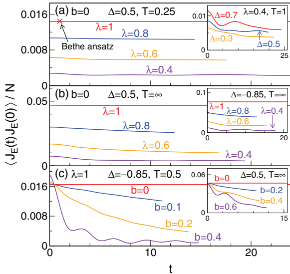
FIG. 2. (Color online) Linear-response energy current correlation function whose long-time asymptote determines the Drude weight through Eq. (9). For the integrable XXZ chain ( \lambda = 1 , b = 0 ), the global energy current J_E = \sum_n J_E(n) is conserved; thus \langle J_E(t)J_E \rangle = \langle J_E(0)J_E \rangle , and DMRG can be compared with exact Bethe ansatz results (symbol). (a) and (b) Nonintegrable dimerized chain. The current correlation function seems to saturate at a finite value (or decays on a hidden large temperature-independent time scale), indicating a finite Drude weight D > 0 . (c) The data in presence of a staggered field b > 0 are consistent with D = 0 .
