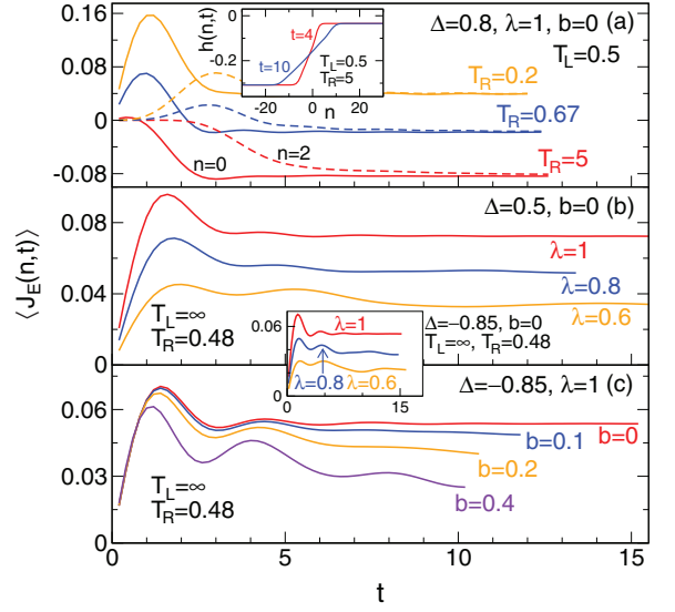
FIG. 1. (Color online) Energy current flowing between two semi-infinite spin-1/2 chains, which are initially in thermal equilibrium at different temperatures T_{L,R} and coupled at time t = 0 and position n = 0 . (a) Integrable XXZ chain with z anisotropy \Delta . The behavior in the gapped phase \Delta > 1 is similar. (b, lower inset) Nonintegrable dimerized XXZ chain where the coupling on every second bond is reduced by \lambda . The latter is irrelevant at \Delta = -0.85 but opens a gap for \Delta = 0.5 . (c) XXZ chain in presence of a staggered field b rendering the model nonintegrable. A gap opens around b \approx 0.3 . Despite the fact that the local energy density h(n,t) does not relax (upper inset), the current saturates fast to a unique finite value except for b > 0 . We attribute this to a finite linear-response thermal Drude weight of both the pure XXZ chain and the nonintegrable dimerized chain (see Fig. 2).
