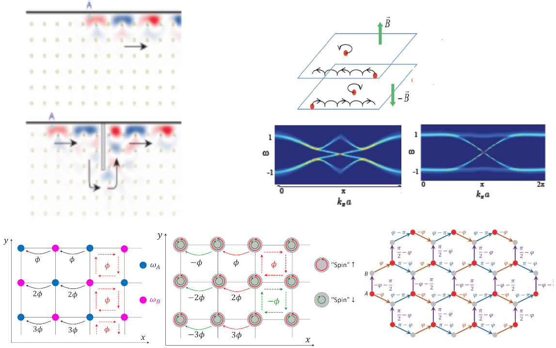
FIGURE 5 : Top : Left, first experimental observation of chiral edge modes and quantum Hall phases of photons in gyromagnetic photonic crystals [67, 74]. Bottom, Left : possible Floquet scheme suggested in Ref. [318] to realize Peierls phases and quantum Hall phases for photon systems without the Faraday effect. Bottom, middle : Generalization to a quantum Spin Hall state, as observed experimentally in silicon photonics at University of Maryland [69, 70]. Top, right : Spectral function from Ref. [332] computed with CDMFT [336, 337] exemplifying that the helical edge modes of the Kane-Mele model are robust towards interaction effects. Bottom, right : Possible phase configuration using the Floquet scheme of Eq. (17) producing an Haldane state with anisotropic couplings (see Eq. (19)).
