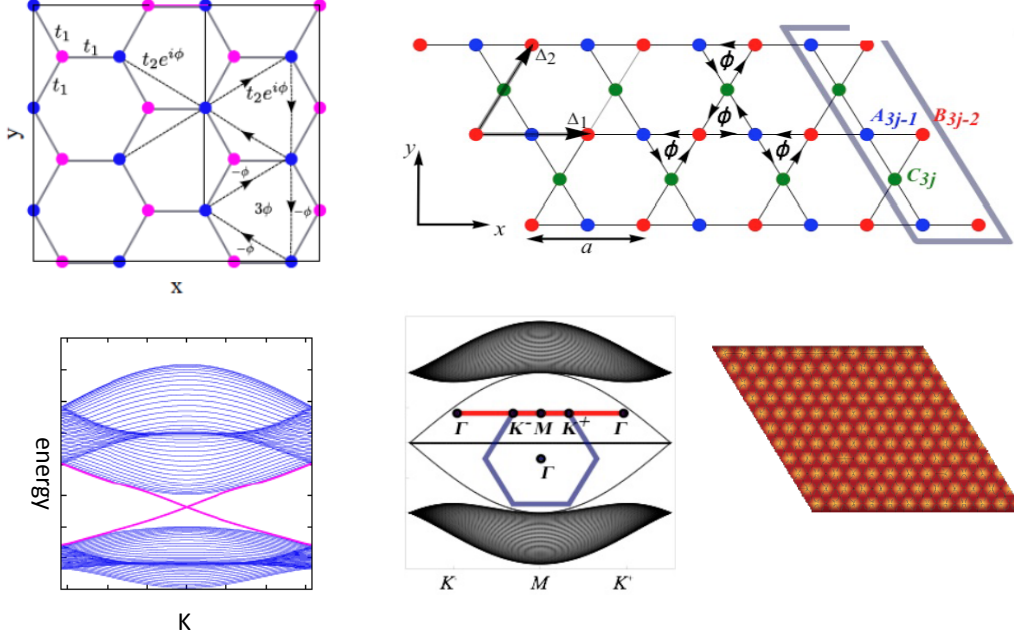
FIGURE 4 : Left : Representation of the Haldane model on the honeycomb lattice [287] (top) and spectrum of the system in the topological phase (bottom). Right : Kagome lattice with artificial fluxes [59], dual to the honeycomb lattice with Josephson junction rings introduced in Ref. [56]. This can be seen as a realization of the Haldane model on the Kagome lattice with no net flux on a parallelogram unit cell. Bottom, middle : spectrum of the Kagome lattice for one particular flux configuration \phi = \pi/6 (with the notations of Ref. [59]), showing a flat band in the middle of the energy spectrum in addition to chiral edge modes. Right, the local density of states then also shows states trapped on hexagonal cells [59], as observed in the experimental setup of Ref. [98].
