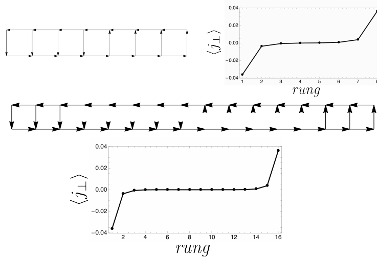
FIGURE 6 : DMRG and Exact Diagonalization results on small ladders with bosons, with 8 and 16 rungs, showing that the Meissner currents subsist in a Mott phase with total density 1, as predicted by the theory [365, 366]. Here, the parameters are fixed to : formally U \rightarrow +\infty (hard-core bosons), V_{\perp} = 4t , t = 1 , t_{\perp} = 1 and the flux is fixed to \chi = \pi/25 using the notations of Ref. [366]. Other careful DMRG analyses of this model have been performed in Refs. [367, 368, 369].
