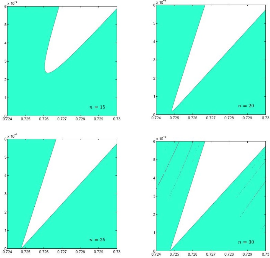
FIGURE 5. The sets \{(E, V) : E \in \Sigma_V^{(n)}\} near (0.7248, 0) for n = 15, 20, 25, 30 .
