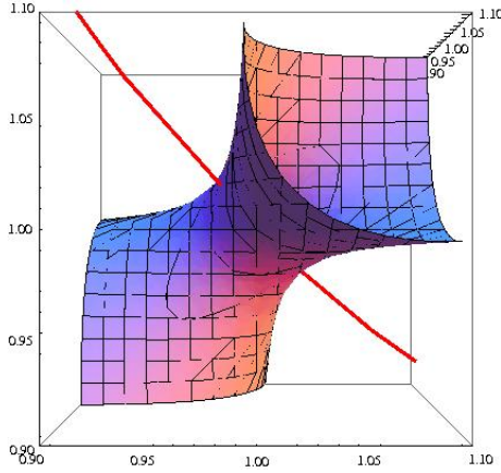
FIGURE 7. S_{0,1} and Per_2(T) near (1, 1, 1) .
