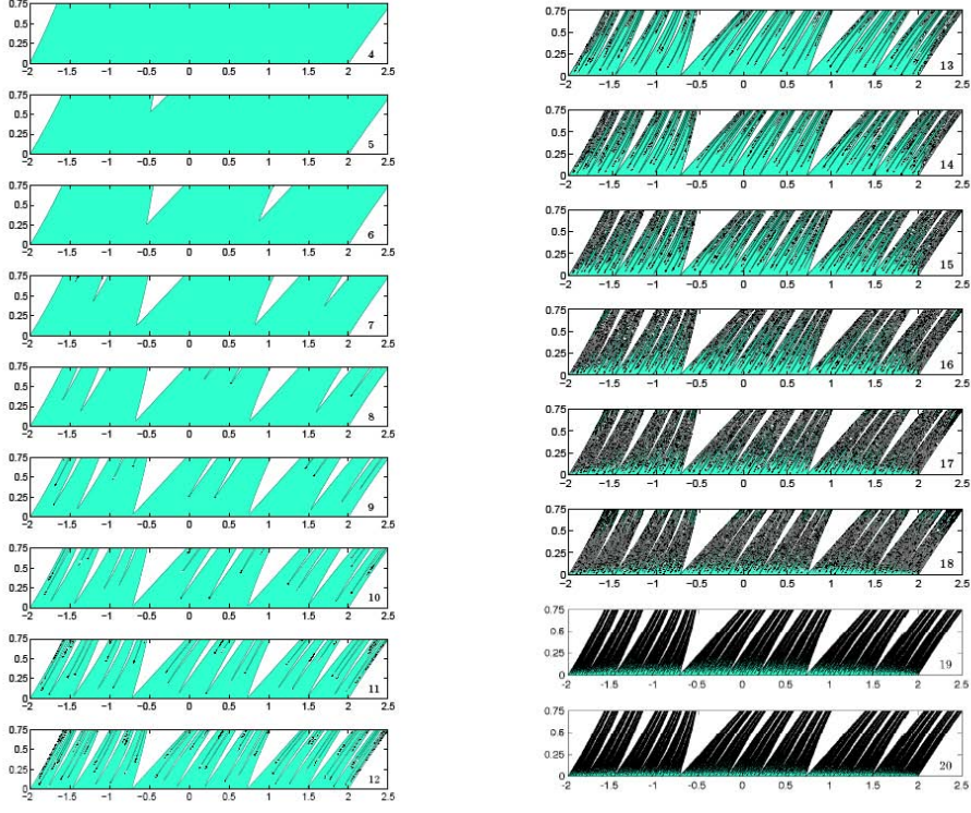
FIGURE 4. The sets \{(E, V) : E \in \Sigma_V^{(n)}, 0 \leq V \leq \frac{3}{4}\} through n = 20 .
