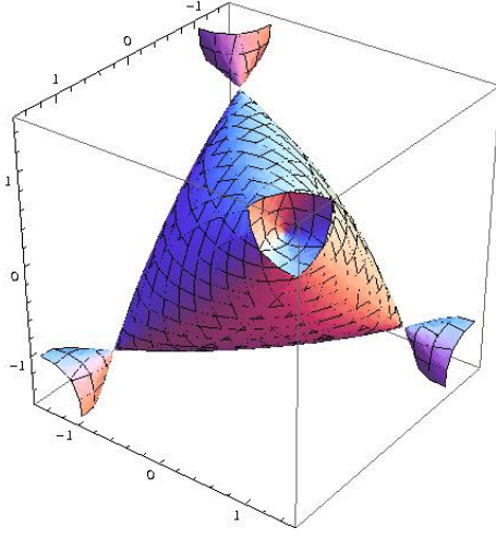
FIGURE 2. The surface S_{0.01} .
