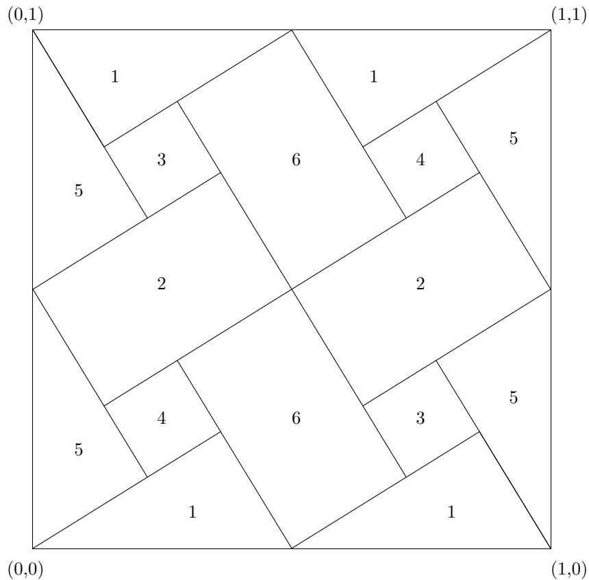
FIGURE 6. The Markov partition for the map \mathcal{A} .
