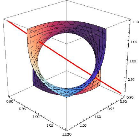
FIGURE 8. S_{0,2} and Per_2(T) near (1, 1, 1) .
