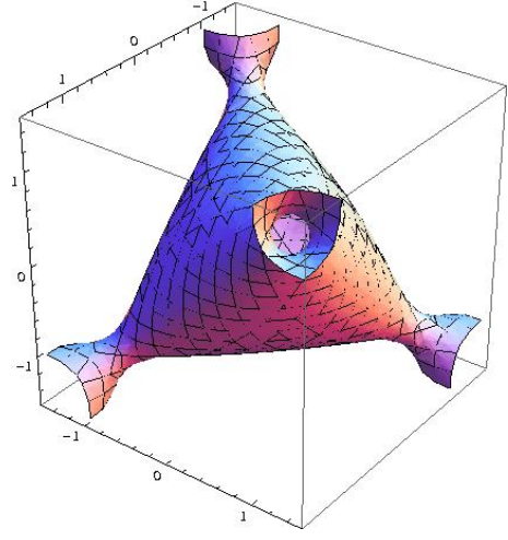
FIGURE 3. The surface S_{0.5} .
