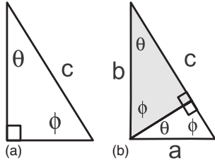
Fig. 1. (a) A right triangle specified by the angles \{\theta, \phi\} and hypotenuse c . (b) The same triangular area can be described by two similar triangles of hypotenuses a and b .
