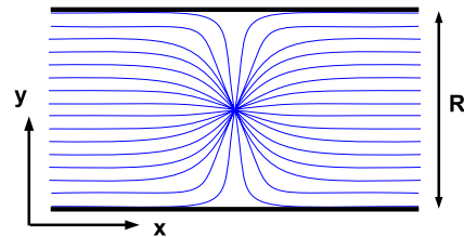
Fig. 3. Electric field of a point charge confined in one infinite dimension ( x ) and one finite dimension ( y ) of scale R .
