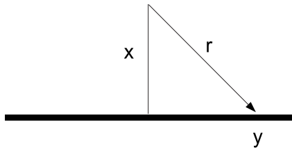
Fig. 2. Coordinate system for an infinite line of charge running in the y -direction with linear charge density \lambda = dQ/dy . We calculate the potential V(x) at a fixed perpendicular distance x from the line of charge. The distance to the element of charge dQ is r = \sqrt{x^2 + y^2} .
