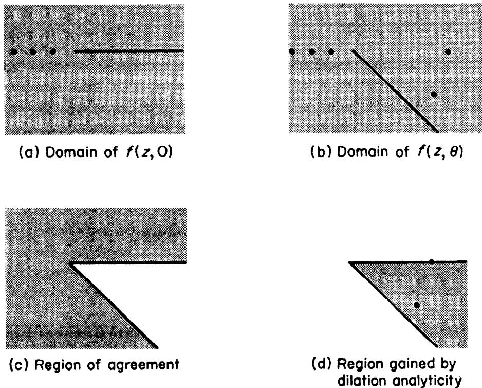
FIGURE XIII.5 Analytic continuation of matrix elements of the resolvent.
