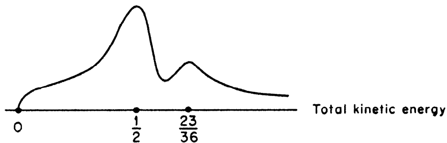
FIGURE XII.3 Schematic elastic scattering cross section for e + \text{He}^+ \rightarrow e + \text{He}^+ .
