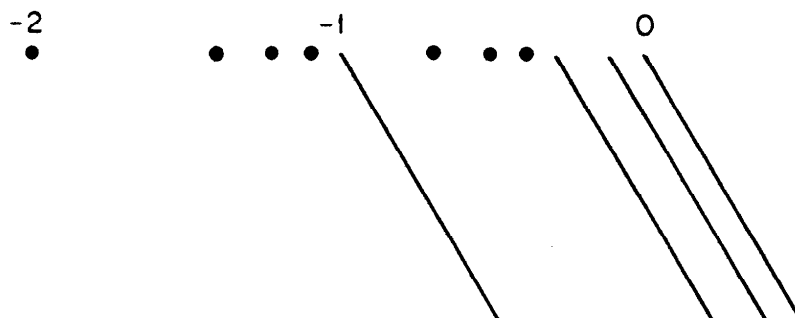
FIGURE XII.8 \sigma(H_0(\theta)) .
