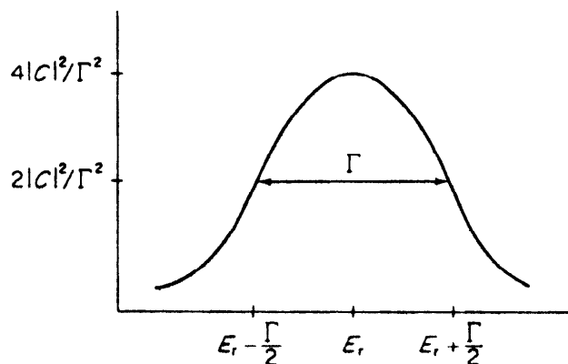
FIGURE XII.6 A Breit-Wigner resonance shape.
