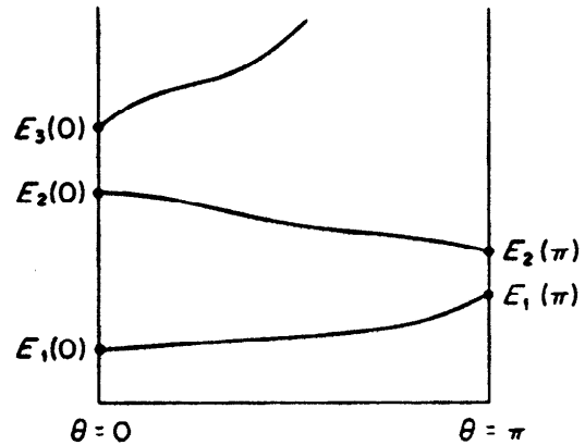
FIGURE XIII.13 Bands in one-dimensional Schrödinger operators.
