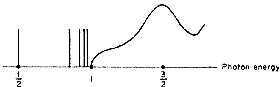
FIGURE XII.4 Schematic absorption cross section for \text{He} + \gamma .
