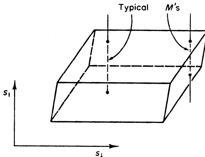
FIGURE XIII.17 The s decomposition of \tilde{Q} .
