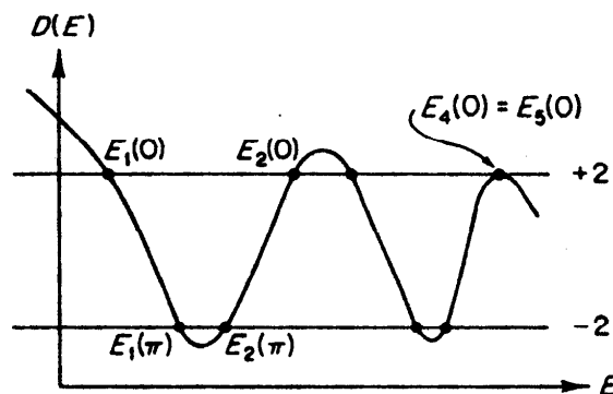
FIGURE XIII.14 A typical discriminant.
