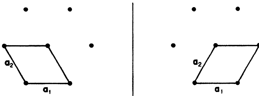
FIGURE XIII.18 Two choices of basis and basic cell.
