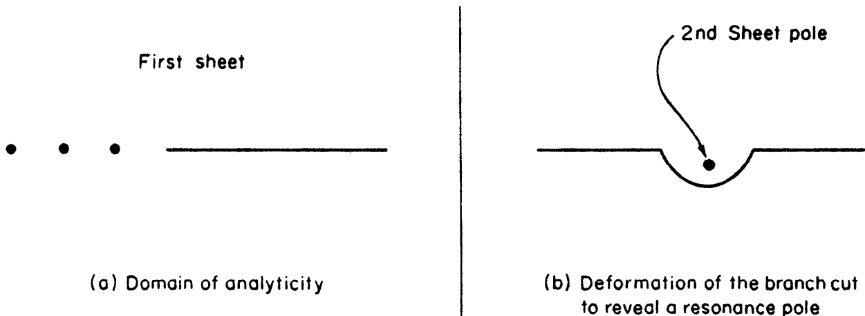
FIGURE XII.5 Continuation of the scattering amplitude.
