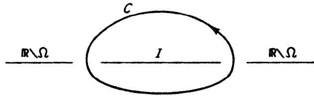
FIGURE XIII.4 A contour of integration.
