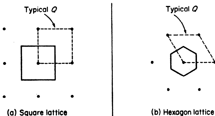
FIGURE XIII.19 Two Wigner–Seitz cells.
