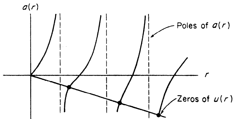
FIGURE XIII.1 The Riccati function a(r) .
