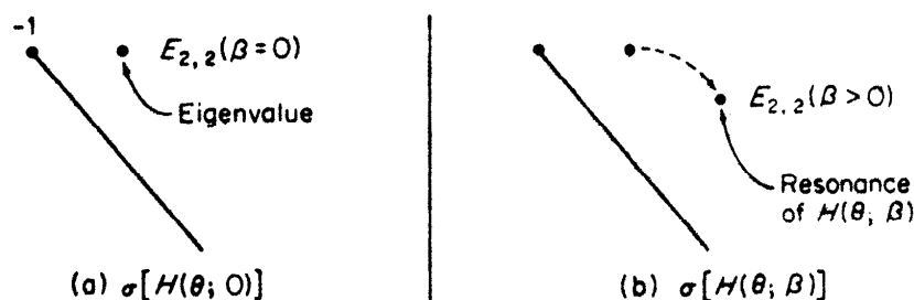
FIGURE XII.9 Trajectory of E(\beta, \theta) for \theta fixed; \text{Im } \theta > 0 .
