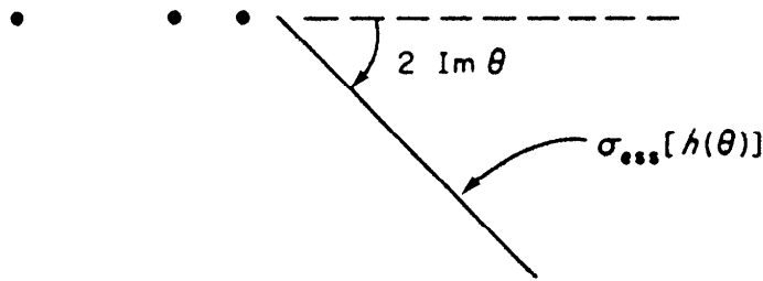
FIGURE XII.7 \sigma(h(\theta)), 0 \leq \text{Im } \theta \leq \pi/2 .
