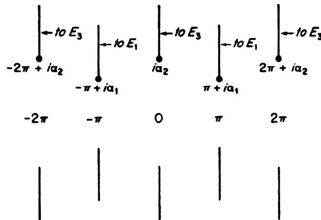
FIGURE XIII.16 The Riemann surfaces of an energy band; n = 2 .
