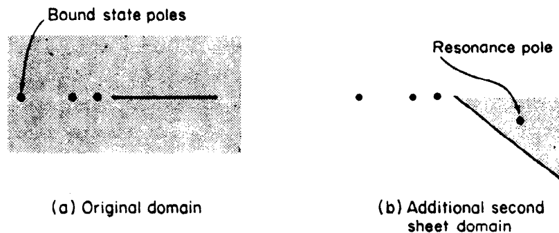
FIGURE XII.10 Domain of analyticity for R_\psi(E) .
