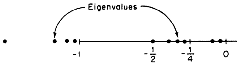
FIGURE XII.2 The spectrum of H_0 .
