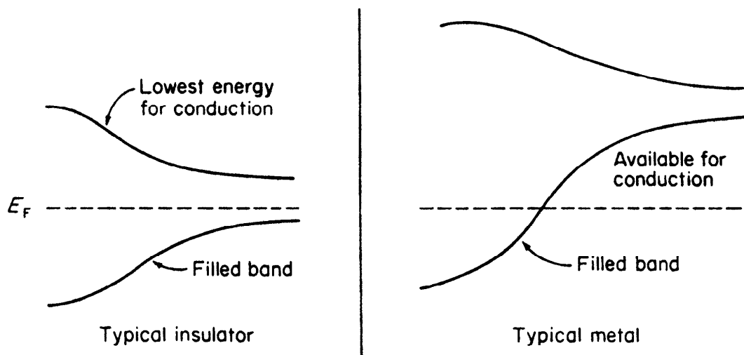
FIGURE XIII.20 Energy bands in conductors and insulators.
