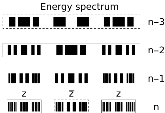
Figure 4: Spectrum of the approximant H_n ( n = 8 ) constructed geometrically from the spectra of H_{n-2} and H_{n-3} (relation (4)). z and \bar{z} are the two scaling factors.
