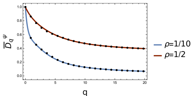
Figure 15: The averaged fractal dimensions of the wavefunctions D_q^\psi as a function of the multifractal parameter q , for \rho = 0.1, 0.5 . Dots: numerical results, solid line: theoretical predictions.
