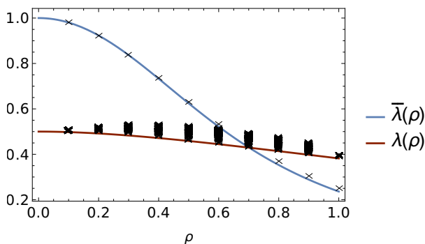
Figure 12: Numerical results and theoretical predictions for the renormalization factors \bar{\lambda}(\rho) and \lambda(\rho) . Dots: Numerical results ( n = 19 , 4181 sites). Solid lines: theoretical predictions (32).
