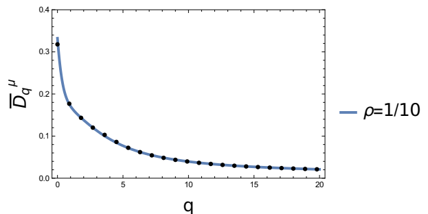
Figure 16: The averaged local spectral dimensions D_q^\mu as a function of the multifractal parameter q , for \rho = 0.1 . Dots: numerical results, solid line: theoretical predictions (eq. (39)).
