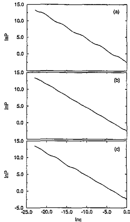
Figure 2. Scaling behaviour of the DOS measure of the Fibonacci chain for the off-diagonal model with t_A = 1 , t_B = r_c \simeq 10.6 : (a) E = 0 ; (b) E = E_{1111\dots} = 11.17942667\dots ; (c) E = E_{11110000\dots} = 11.17942509\dots
