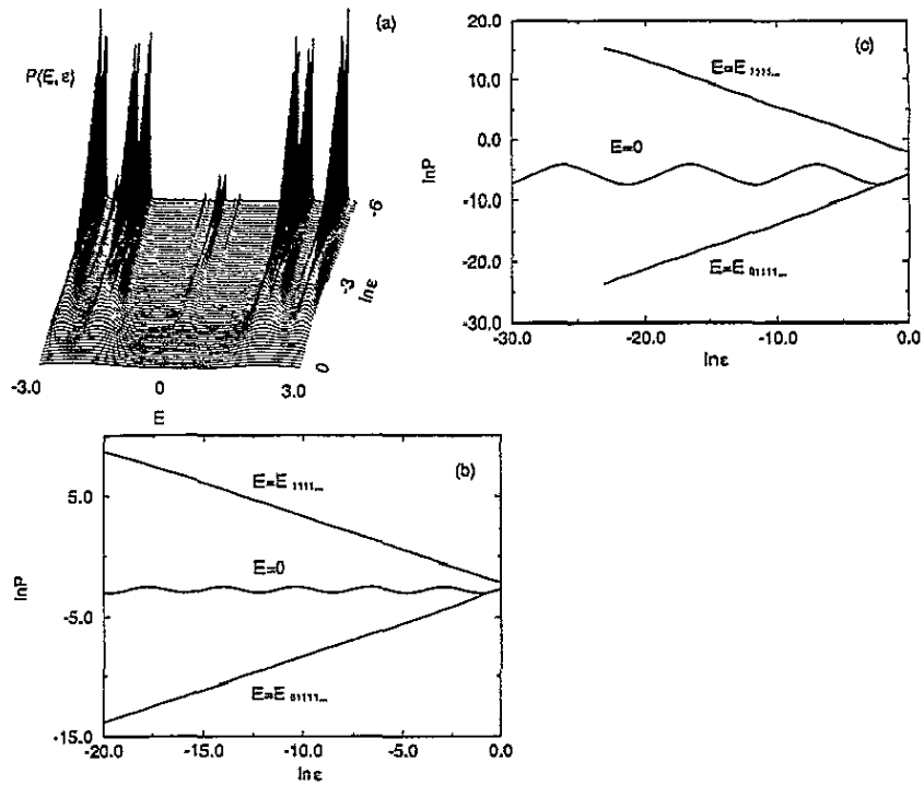
Figure 3. Scaling behaviour of the LDOS measure at the site corresponding to the transformation T_A : (a) plot of P(E, \epsilon) for t_A = 1, t_B = 2 ; (b) \ln P(E, \epsilon) against \ln \epsilon at eigenenergies E = 0, E = E_{1111\dots} = 2.83395643\dots and E = E_{01111\dots} = 0.47916281\dots for t_A = 1, t_B = 2 ; (c) \ln P(E, \epsilon) against \ln \epsilon at eigenenergies E = 0, E = E_{1111\dots} = 11.17942667\dots and E = E_{01111\dots} = 0.09775744\dots for t_A = 1, t_B = r_c = 10.6 .
