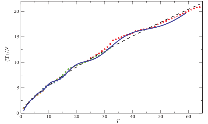
FIG. 1. (Color online) Plot of the spatial dependence of the MFPT observable \langle \mathbf{T} \rangle / N , as a function of the source-target distance r , for the Sierpinski gasket. The dotted points are numerical data (gaskets of generation 3, 4, 5, 6, respectively in yellow, blue, green, red), the dashed black line is the leading behavior r^{d_w - d_f} , as studied in Refs. [2,3]. The blue solid line is a more refined fit from (14) with b_2 = 0.05 , and \phi = \pi/2 .
