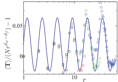
FIG. 2. (Color online) Plot of the corrections to the leading r^{d_w - d_f} behavior of the spatial dependence of the MFPT \langle \mathbf{T} \rangle / N , as a function of the source-target distance r , for the Sierpinski gasket. Circles stand for numerical simulations (gaskets of generation 3, 4, 5, 6, respectively in black, red, green, blue), and the blue solid line is a fit from (14). This figure clearly shows the log-periodic oscillations with the variable 2\pi \ln r / \ln l .
