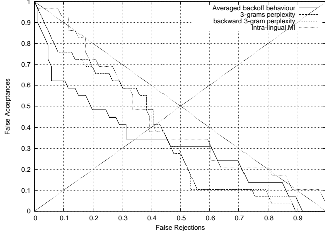
Figure 5. DET curves of 3-gram, backoff and intra-lingual mutual information based confidence measures at sentence level
