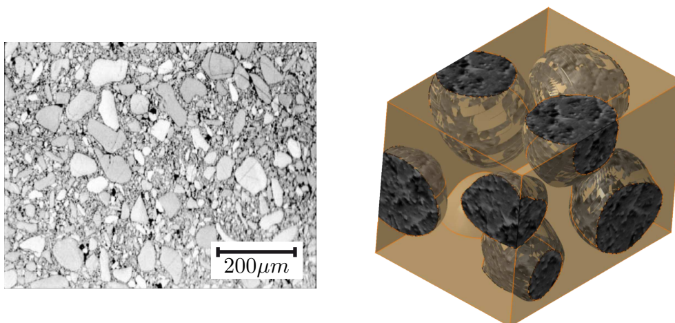
Figure 5.19: Micrographie et architecture grains/matrice ( Image CEG )
