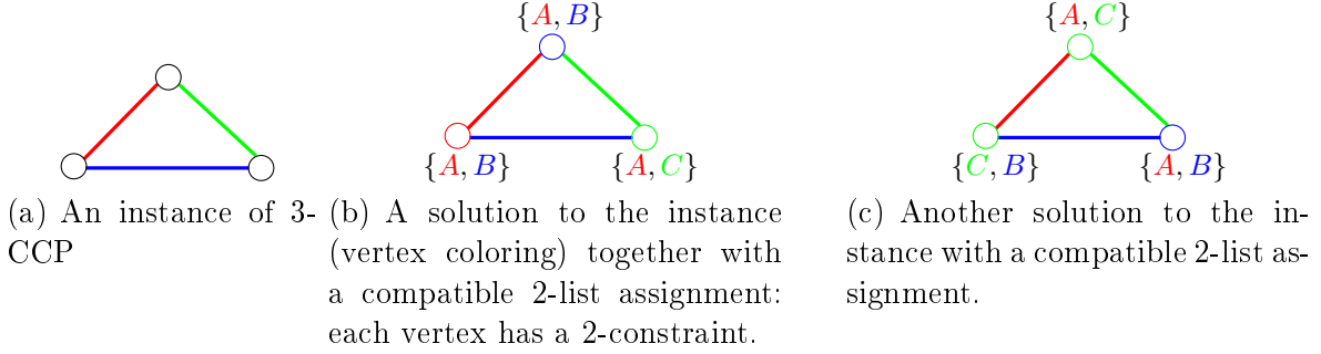
Figure 4: Illustration of definitions. Color correspondence: A=red ; B=blue ; C=green. Both 2-list assignments together form a 2-list covering because any solution is compatible with at least one of them.
