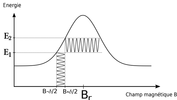
FIGURE 13 – Modulation d'amplitude
