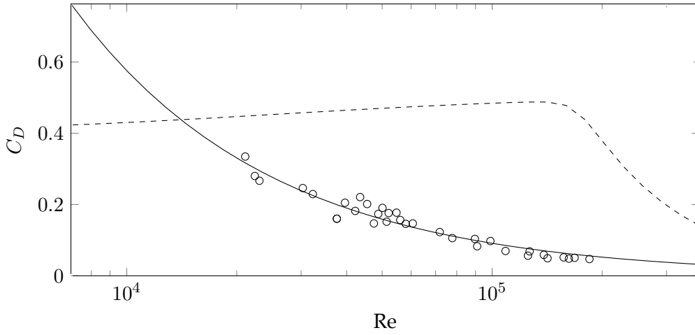
Figure 9.2: The drag coefficient for an Iridaea flaccida . “○” represents the experimental values given in Gaylord et al. (1994), “—” represents the best fit line of those values and “---” represents the empirical formula for a sphere given by Almedeij (2008).
