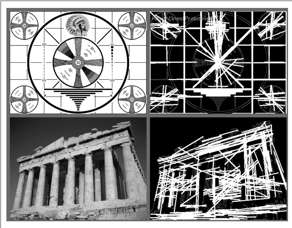
Figure 6-11. The Canny edge detector ( \text{param1}=50 , \text{param2}=150 ) is run first, with the results shown in gray, and the progressive probabilistic Hough transform ( \text{param1}=50 , \text{param2}=10 ) is run next, with the results overlaid in white; you can see that the strong lines are generally picked up by the Hough transform
