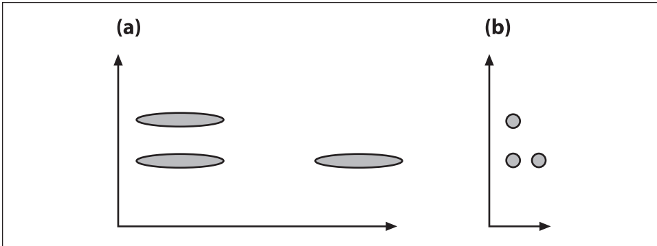
Figure 13-4. The Mahalanobis computation allows us to reinterpret the data's covariance as a "stretch" of the space: (a) the vertical distance between raw data sets is less than the horizontal distance; (b) after the space is normalized for variance, the horizontal distance between data sets is less than the vertical distance
