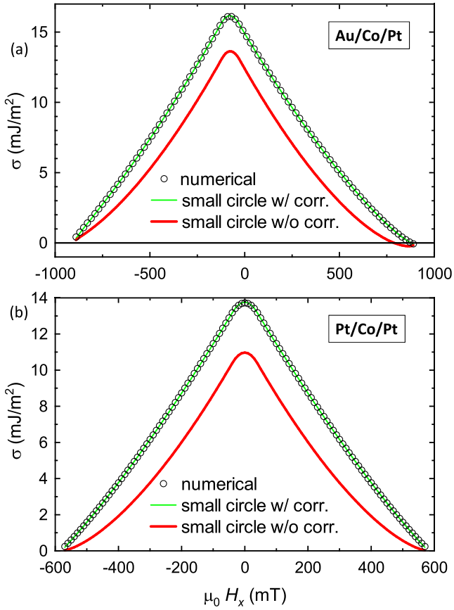
Fig. 7. Comparison of the small circle model with numerical simulations, for the Au/Co/Pt (a) and Pt/Co/Pt (b) samples, regarding the domain wall energy. The effect of the analytical domain wall energy correction (see Appendix) is shown. For Au/Co/Pt, the domain wall energy maximum is reached at \mu_0 H_x = -75 mT.
