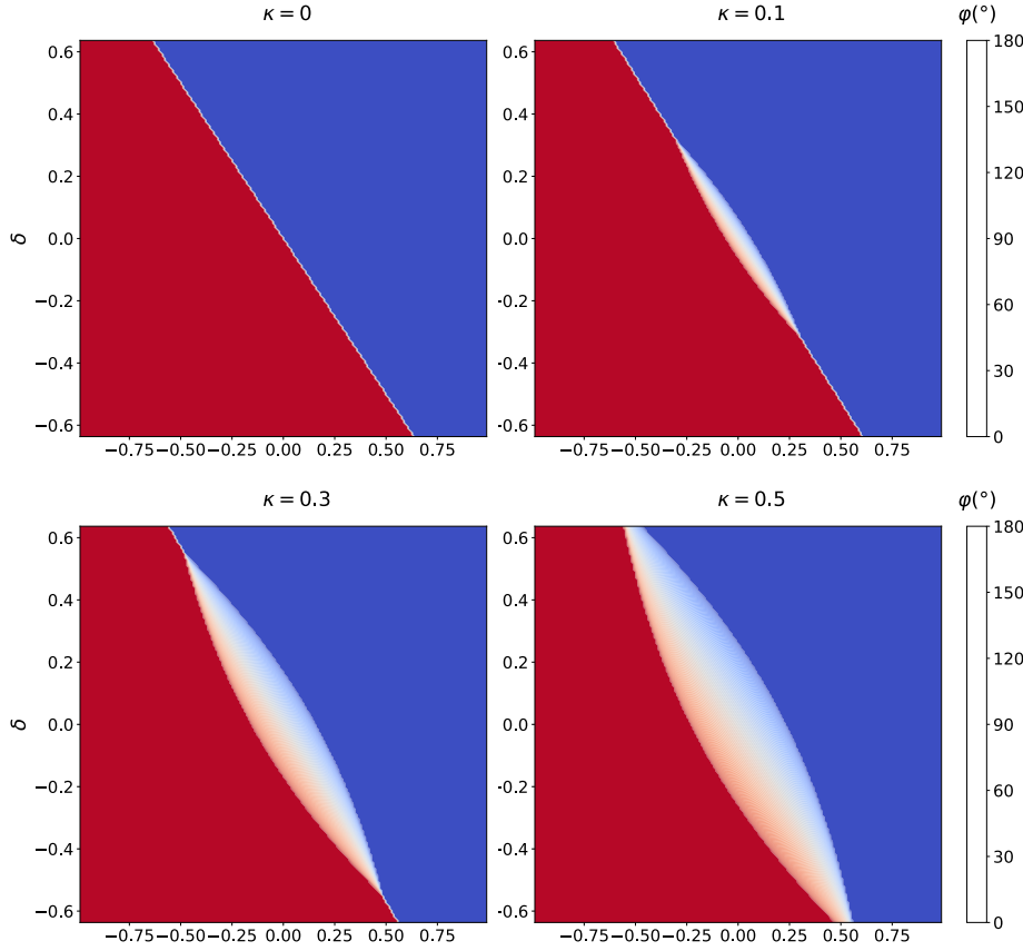
Fig. 4. Type of domain wall as a function of in-plane field (scaled field h ) and DMI (expressed by the scaled parameter \delta ), for increasing values of the domain wall magnetostatic energy (scaled parameter \kappa ). For these drawings, a fixed direction in the plane is considered, so that negative fields are figured, and \varphi spreads over the [0, \pi] interval. The color code represents the cut angle \varphi , plotted over the extended range from 0 to \pi so as to differentiate the two chiralities of Néel walls. The constrained model predicts a switching at h = -\delta , the \phi iso-values being parallels to that line.
