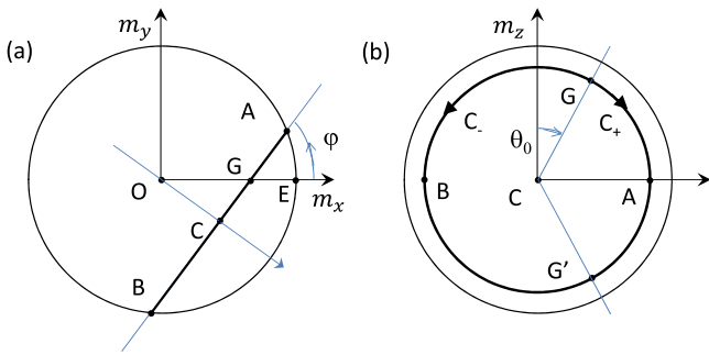
Fig. 1. The ‘small circle’ Ansatz. (a) Top view of the unit sphere for the magnetization vectors, under an in-plane field in the +x direction. Point G depicts the magnetization orientation in the n < 0 domain (and hides point G' which corresponds to the n > 0 domain). A small circle of the unit sphere, that goes through G and G' and is vertical, is defined by the cut angle \varphi , which has to be optimized for each situation. Point C is the center of this small circle. The in-plane angle of the domain wall magnetization, called \psi , is defined by the angle of OA with OE ; it is thus different from \varphi . (b) Side view normal to the small circle, showing the two paths that connect G to G' , either through A (short path C_+ where \theta increases), or through B (long path C_- where \theta decreases). The great circle (radius 1) is also drawn in thin line.
