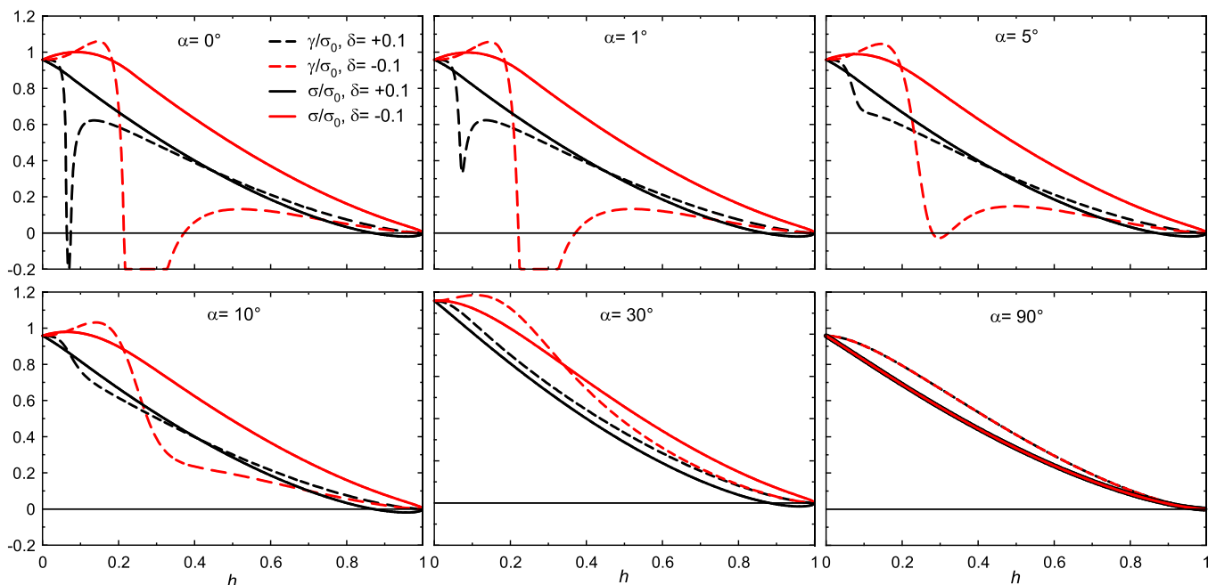
Fig. 9. Results of the numerical minimization using the 'small circle' Ansatz, for a large domain wall relative magnetostatic energy ( \kappa = 0.3 ), for two opposite and small values of the DMI ( \delta = \pm 0.1 ). The domain wall surface energy \sigma (lines) as well as surface tension \gamma (dash lines), normalized to the Bloch wall surface energy \sigma_0 , are plotted as a function of the normalized in-plane field h , for several values of the angle \alpha between the domain wall normal and the applied field.
