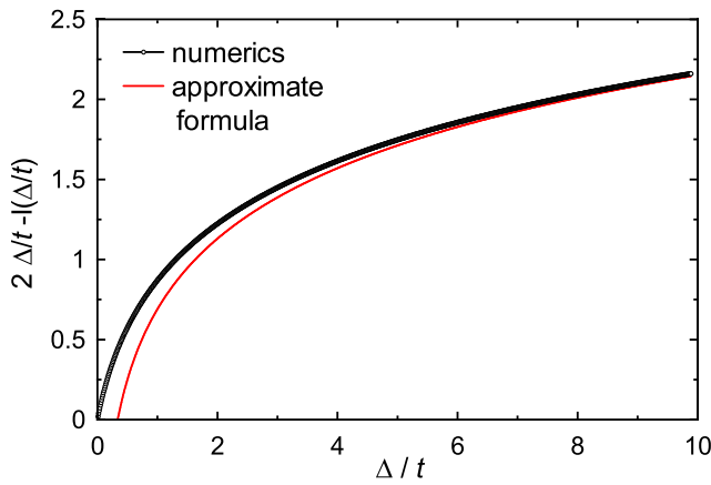
Fig. 15. Numerical evaluation of the function giving the demagnetizing energy correction \sigma_d to the domain wall energy. The large parameter (i.e. \Delta \gg t ) asymptotic behavior 0.69 + 0.635 \ln(\Delta/t) is also drawn.
