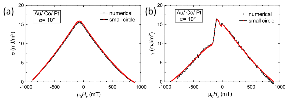
Fig. 12. Comparison of the numerical micromagnetics results (open black symbols) to those of the semi-analytical small circle model (red curves), for the Au/Co/Pt sample. (a) variation of the domain wall energy \sigma with the in-plane field, applied at an angle \alpha = 10 degrees. (b) variation of the domain wall tension \gamma in the same conditions. The analytical correction to the domain wall energy (and tension) is included in the small circle values.
