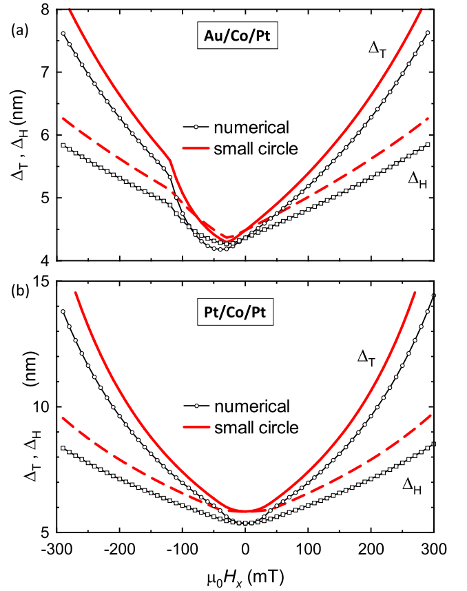
Fig. 8. Comparison of the small circle model with numerical simulations, for the AuCoPt (a) and PtCoPt (b) samples, regarding the domain wall widths (see text for definitions). For AuCoPt, all widths show a minimum at -30 mT for the small circle model, and -40 mT for the numerical calculation, values which are clearly lower from that where the domain wall energy is maximum [see Fig. 7(a)].
