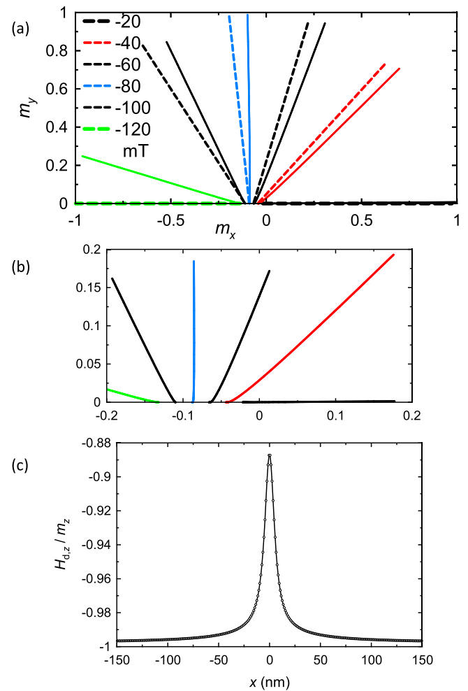
Fig. 6. Comparison of the small circle model with numerical simulations, for the Au/Co/Pt sample. (a) The in-plane magnetization components for an up-down domain wall under several in-plane fields, predicted by the small circle model (dashed lines) and computed by numerical micromagnetics (curves). (b) Zoom close to the origin, for the numerical profiles, to evidence the small deviations from linearity. (c) Profile of the local z demagnetizing factor as extracted from the micromagnetic calculation under zero applied field.
