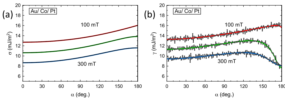
Fig. 11. Comparison of the numerical micro-magnetics results (open black symbols) to those of the semi-analytical small circle model (colored curves), for the Au/Co/Pt sample. (a) variation of the domain wall energy \sigma with angle of the applied in-plane field, for 3 values of the field \mu_0 H = 100, 200, 300 mT. (b) variation of the domain wall tension \gamma in the same conditions. The analytical correction to the domain wall energy (and tension) is included in the small circle values. Note the absence of noise in the semi-analytical calculation of the tension, compared to the numerical procedure (see text for cause).
