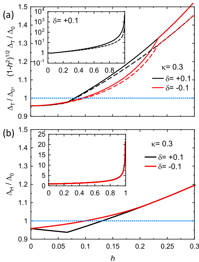
Fig. 5. Results of the numerical minimization using the ‘small circle’ Ansatz, for a large domain wall relative magnetostatic energy ( \kappa = 0.3 ), for two opposite and small values of the DMI ( \delta = \pm 0.1 ). (a) Thiele domain wall width \Delta_T normalized to \Delta_0 , for the small fields. The inset shows the full curve, in log-linear scale. The dashed curves plot the product \sqrt{1-h^2}\Delta_T , the relevant quantity for the domain wall mobility. (b) Hubert domain wall width \Delta_H , normalized to \Delta_0 , the inset showing the full curve, this time in lin-lin scale. The breaks of the curves correspond to the fields ( h = 0.0664 for \delta = +0.1 and h = 0.2334 for \delta = -0.1 ) where the domain wall becomes of the Néel type, perfectly parallel to the field [ \varphi = 0 , see Fig. 3(b)]. The constrained model assumes that all widths are constant, equal to \Delta_0 (dotted lines).
