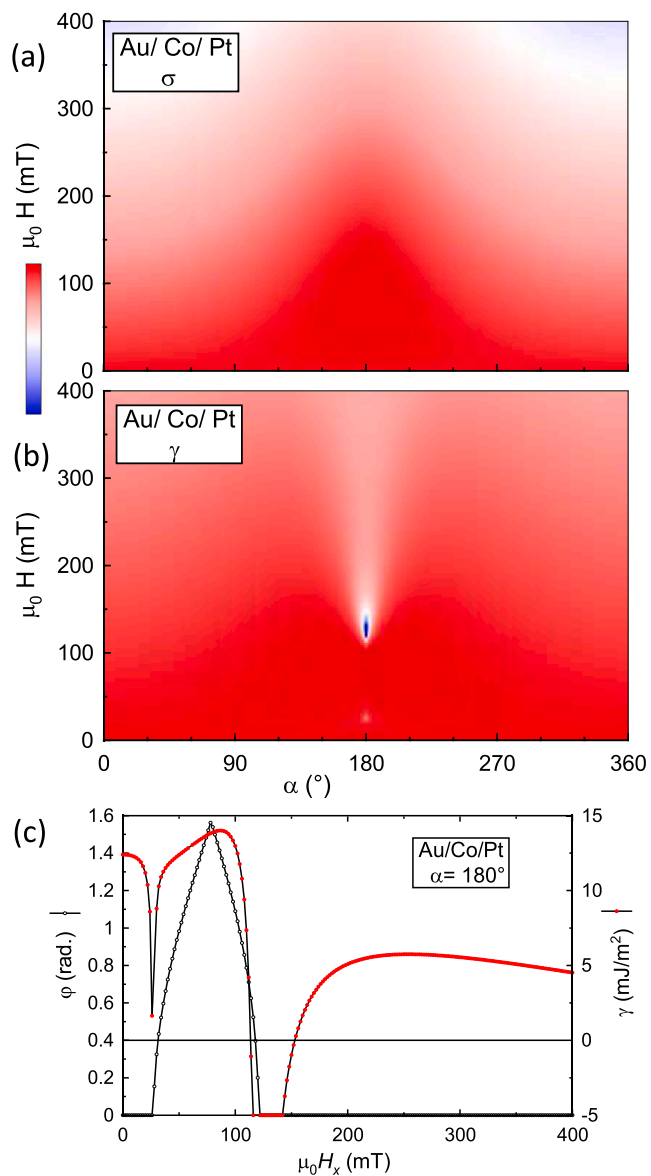
Fig. 13. Computed domain wall surface energy \sigma (a) and tension \gamma (b) for the Au/Co/Pt sample, by the small circle model incorporating the additional demagnetizing energy. Note that such noiseless maps, containing 360x200 pixels, would have required very long numerical micromagnetics calculation times, whereas a few seconds suffice to produce them using the small circle model, including the magnetostatic correction. The color scale spans the values 0 to +14 mJ/m 2 for (a), and -14 to +14 mJ/m 2 for (b), values outside of these boundaries having been clipped. Panel (c) compares a cut of (b) through \alpha = 180^\circ to the variation of the small circle cut angle \varphi .
