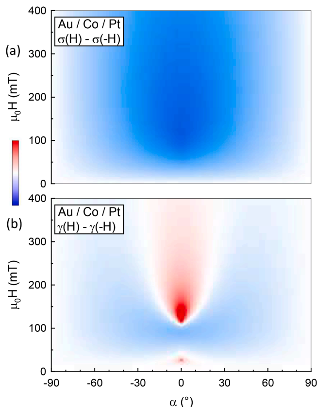
Fig. 14. Computed differences of domain wall surface energy \sigma (a) and tension \gamma (b) for the Au/Co/Pt sample, between positive and negative fields \epsilon(\alpha, H) - \epsilon(\alpha, -H) . The maps are derived from the data of Fig. 13. The color scale spans values -5 to +5 mJ/m 2 for (a), and -10 to +10 mJ/m 2 for (b), values outside of these boundaries having been clipped.
