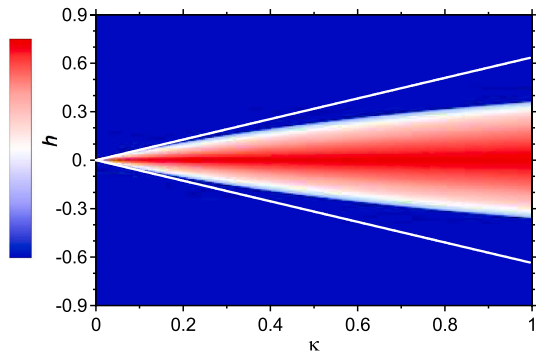
Fig. 2. Results of the numerical minimization using the ‘small circle’ Ansatz, for the case of zero DMI, \delta = 0 . The color code of the map shows the small circle cut angle \varphi , it extends from 0 (blue) to \pi/2 (red). The two lines (also obtained in the constrained model) depict the linear relation valid at small \kappa , see text.
