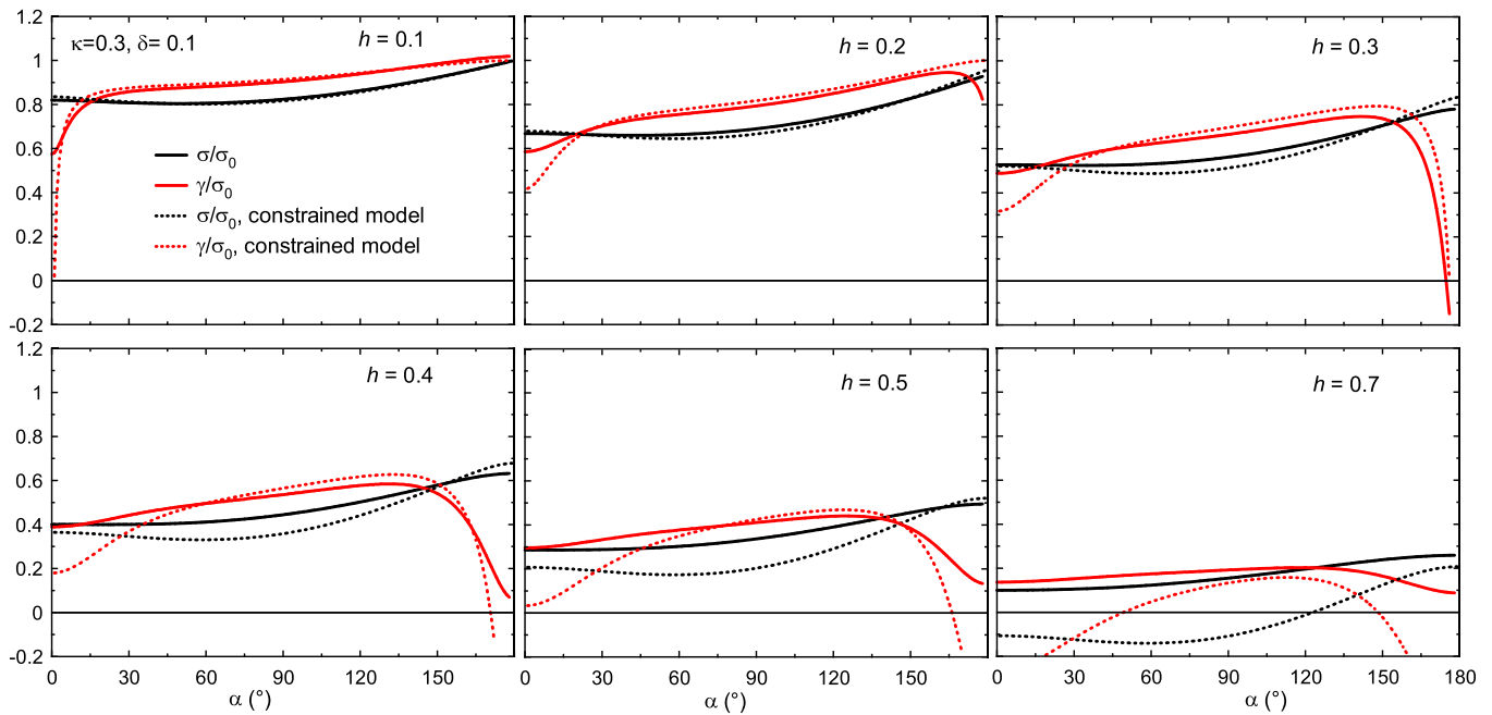
Fig. 10. Alternative view of the results shown in Fig. 9, for \kappa = +0.3 and \delta = +0.1 , where the angle \alpha of the domain wall normal with the in-plane field is varied, for selected values of the field. The results of the constrained model have been included (dotted curves) for comparison.
