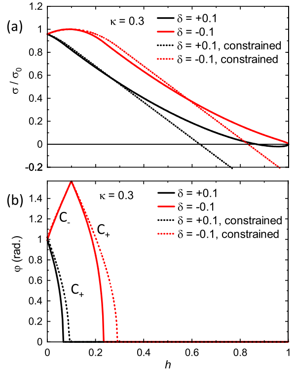
Fig. 3. Results of the numerical minimization using the ‘small circle’ Ansatz, for a large domain wall relative magnetostatic energy ( \kappa = 0.3 ), for two opposite and small values of the DMI ( \delta = \pm 0.1 ). (a) Normalized domain wall energy. The energy maximum in the antiparallel case occurs at h \approx 0.0901 . (b) Corresponding cut angle \varphi , and minimum energy contours C_{\pm} (see Fig. 1). The value \varphi = \pi/2 is reached at h \approx 0.0995 . The zero-field value \varphi \approx 1 radian means that the domain wall is in a mixed Bloch-Néel state with the chosen values of \kappa and \delta . The results of the constrained model are drawn by dotted curves.
