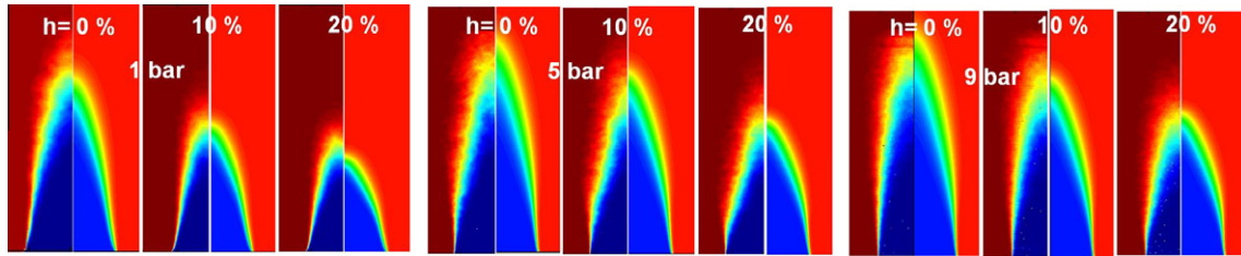
Fig. 7. Orléans Bunsen flames. Comparison between experiment (left) [27], and simulation (right) with the AFSW model and the proposed new model C for the effective Lewis number. Shown are contours of Reynolds averaged progress variable \bar{c} (between 0 and 1) for methane/hydrogen flames with 0, 10, 20 vol.% hydrogen for 0.1, 0.5 and 0.9 MPa ( \phi = 0.6 ).
